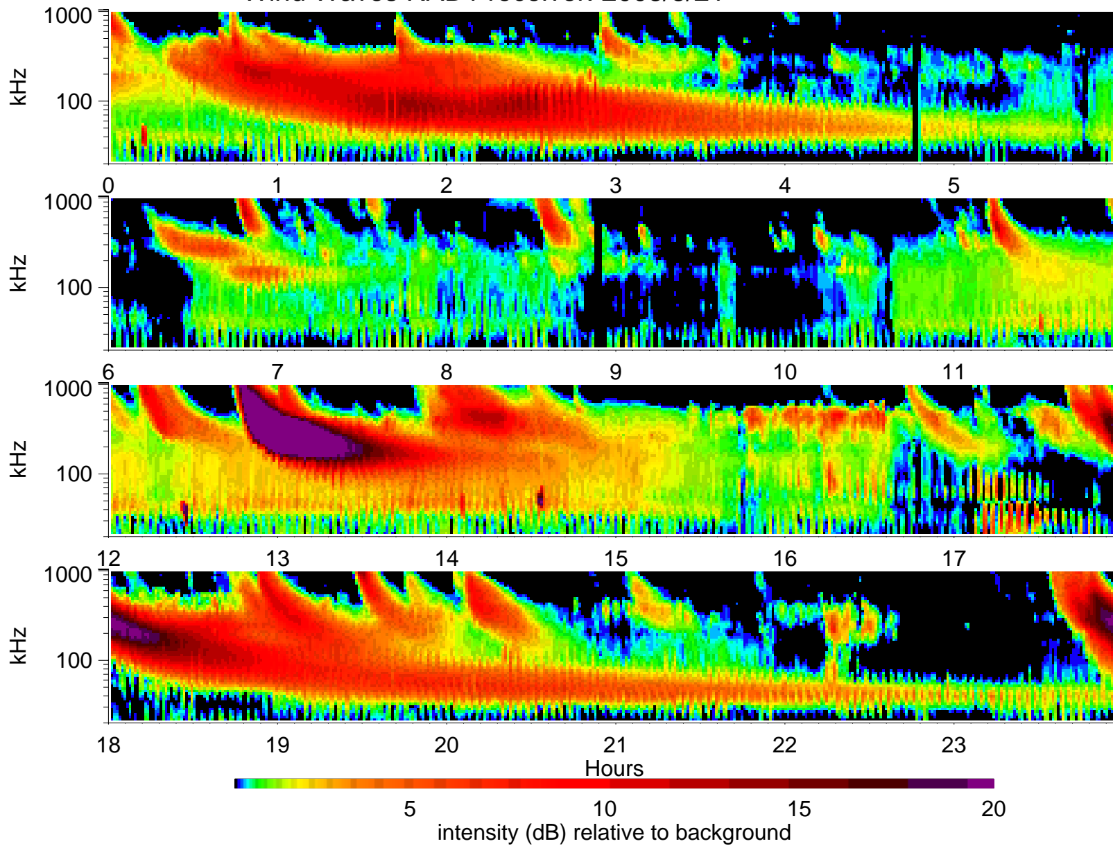
Wind Waves RAD1 receiver: 2003/5/21
