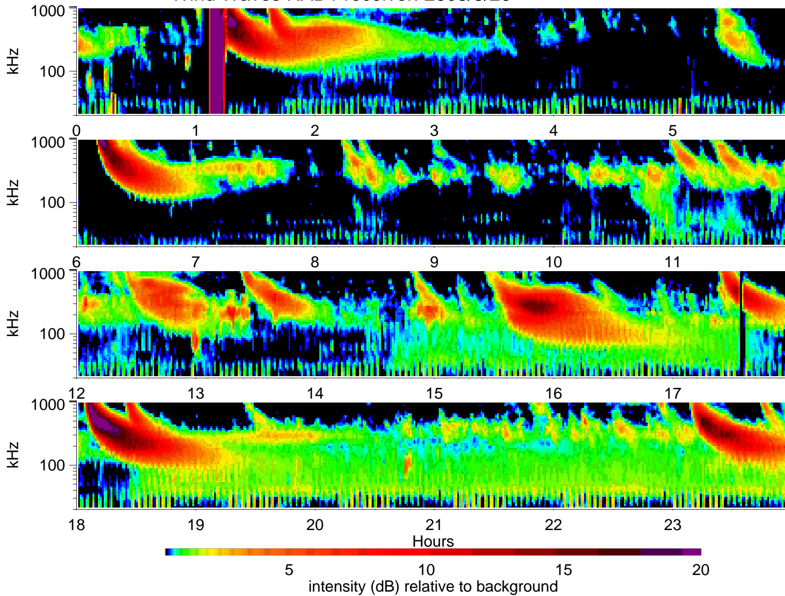
Wind Waves RAD1 receiver: 2003/5/20
