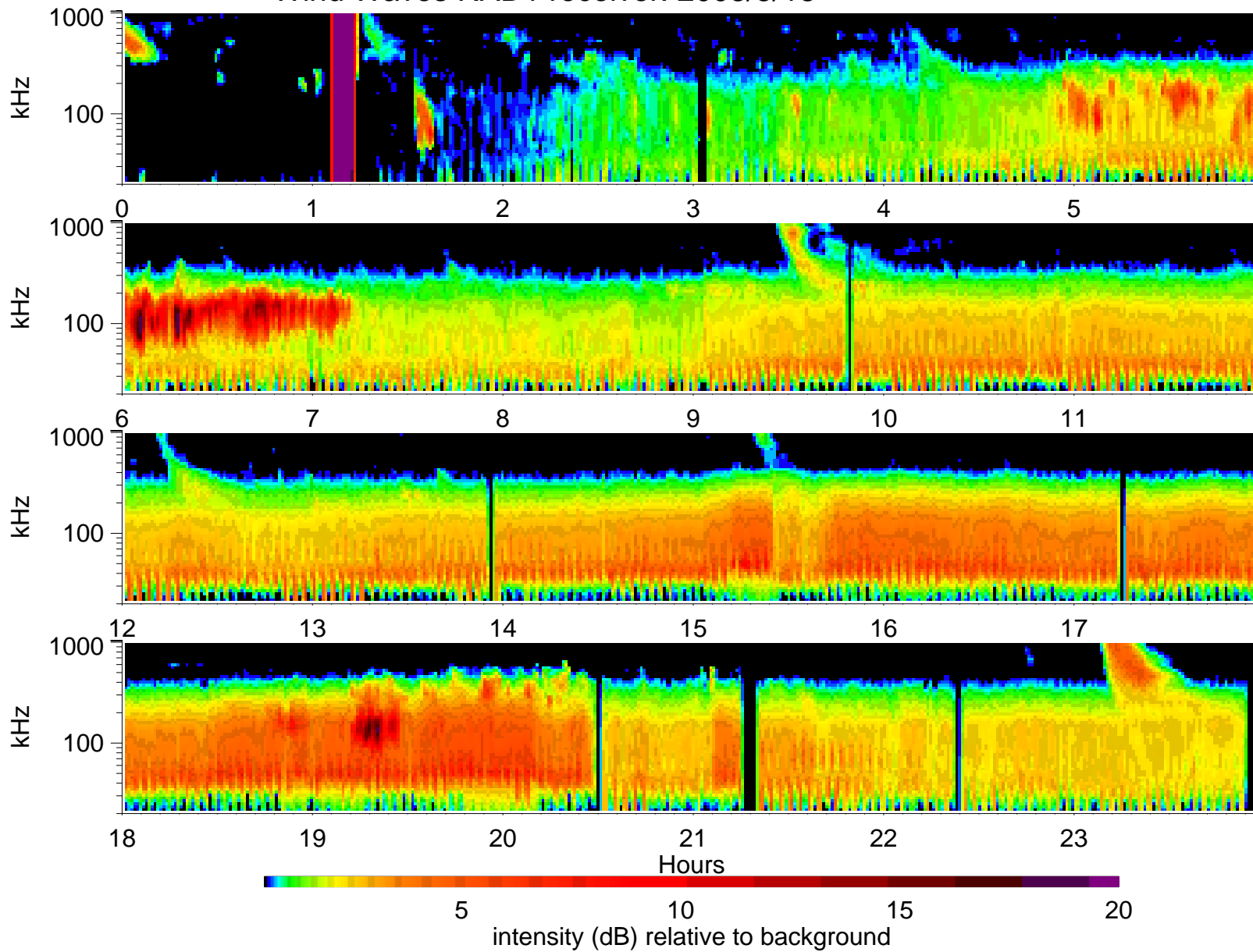
Wind Waves RAD1 receiver: 2003/5/18
