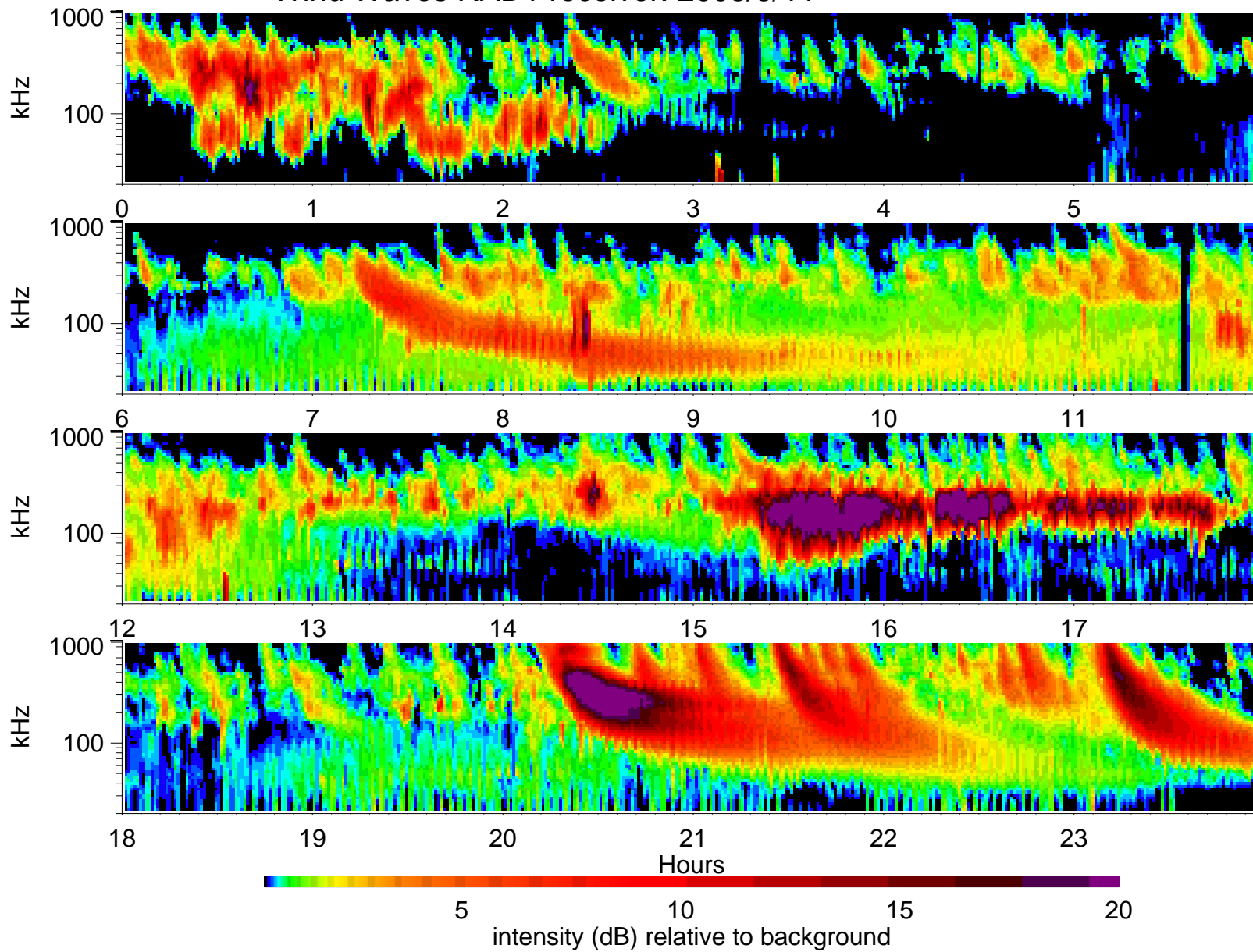
Wind Waves RAD1 receiver: 2003/5/11
