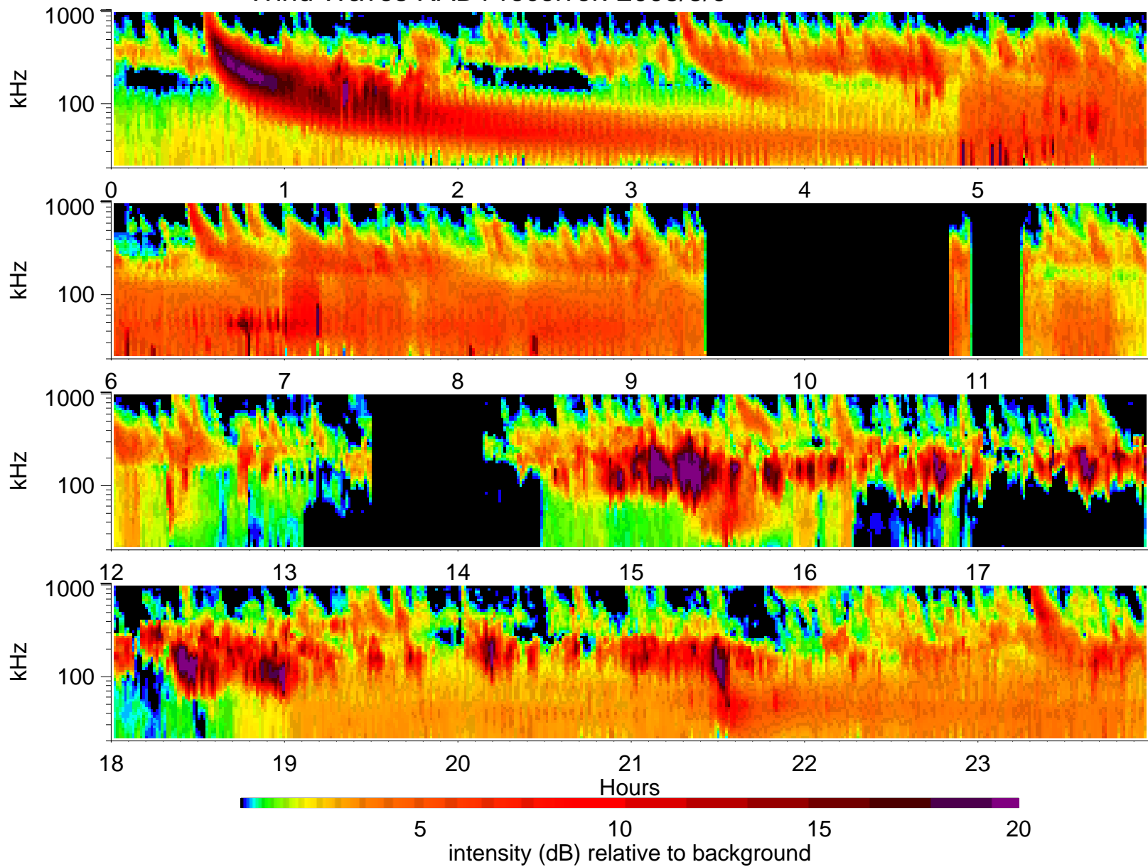
Wind Waves RAD1 receiver: 2003/5/9
