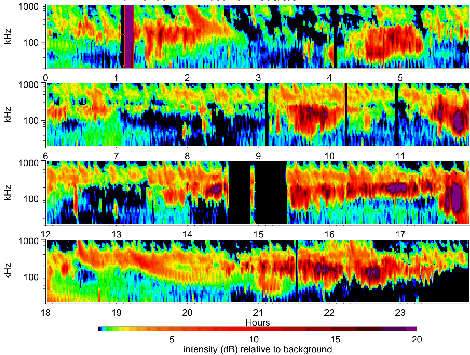
Wind Waves RAD1 receiver: 2003/5/8
