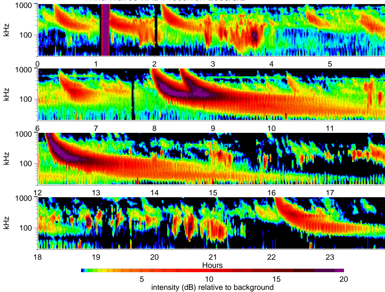
Wind Waves RAD1 receiver: 2003/5/2
