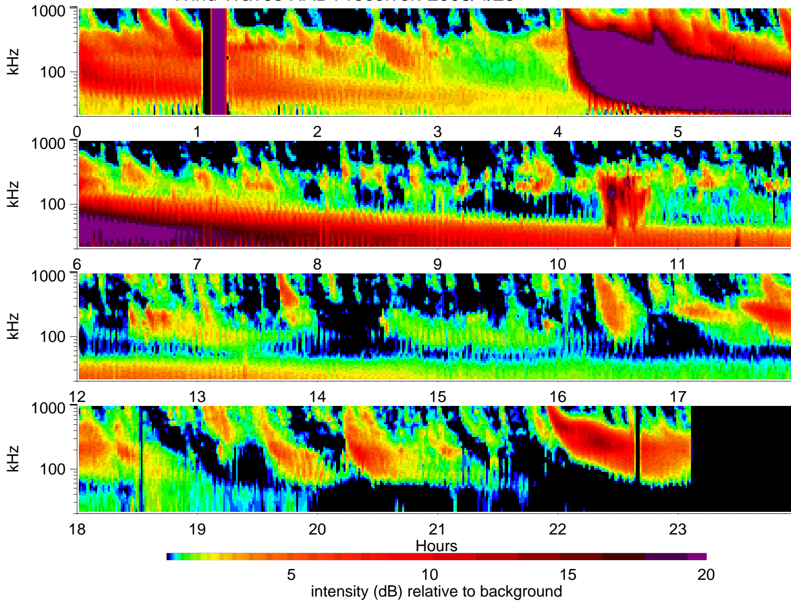
Wind Waves RAD1 receiver: 2003/4/28
