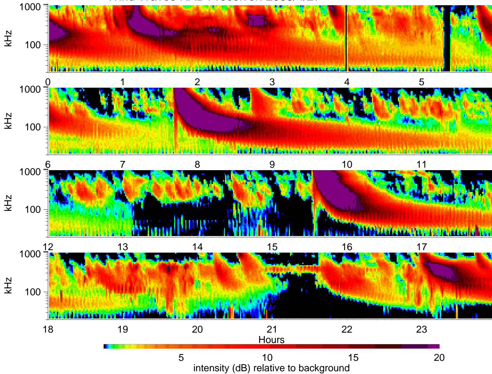
Wind Waves RAD1 receiver: 2003/4/27
