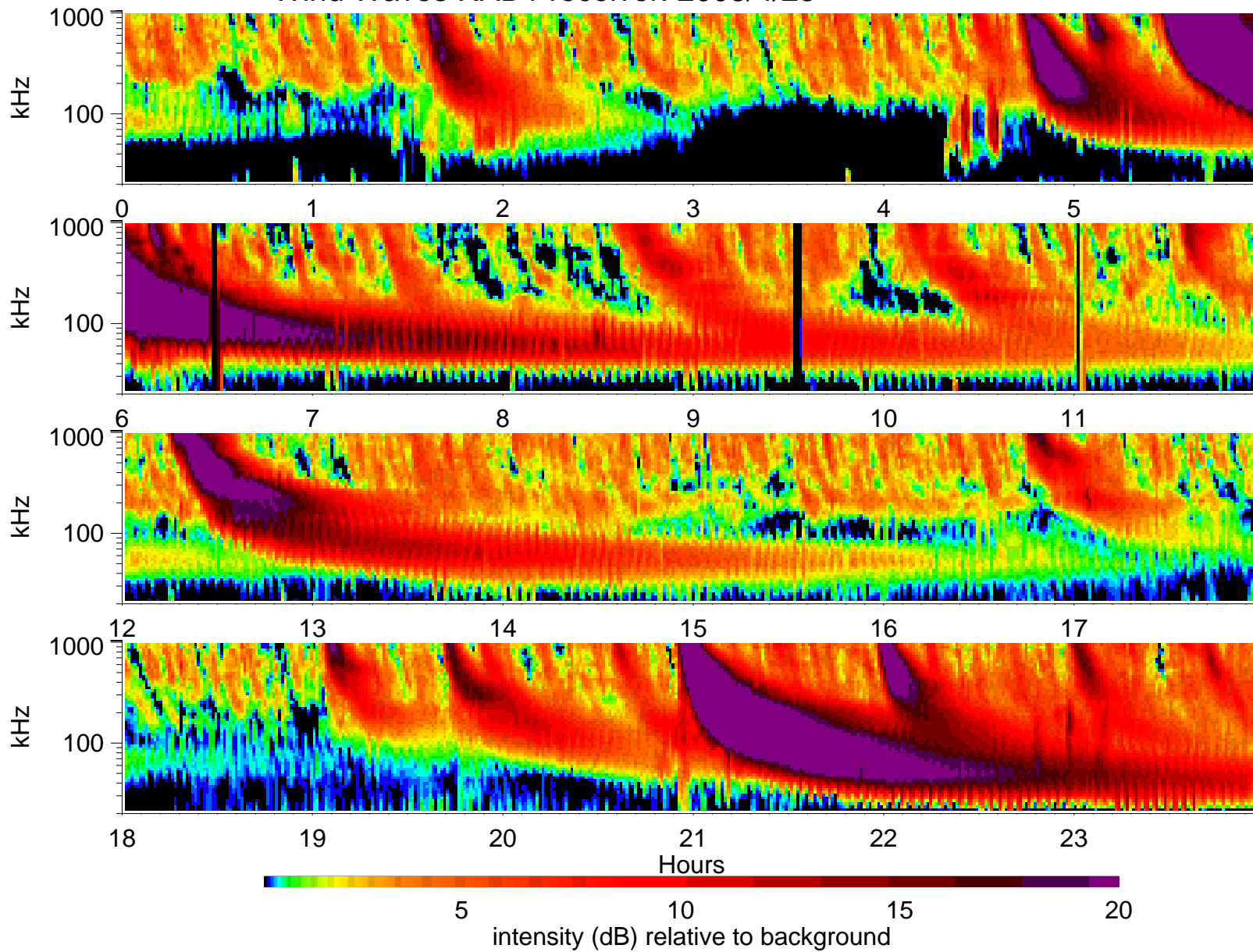
Wind Waves RAD1 receiver: 2003/4/25
