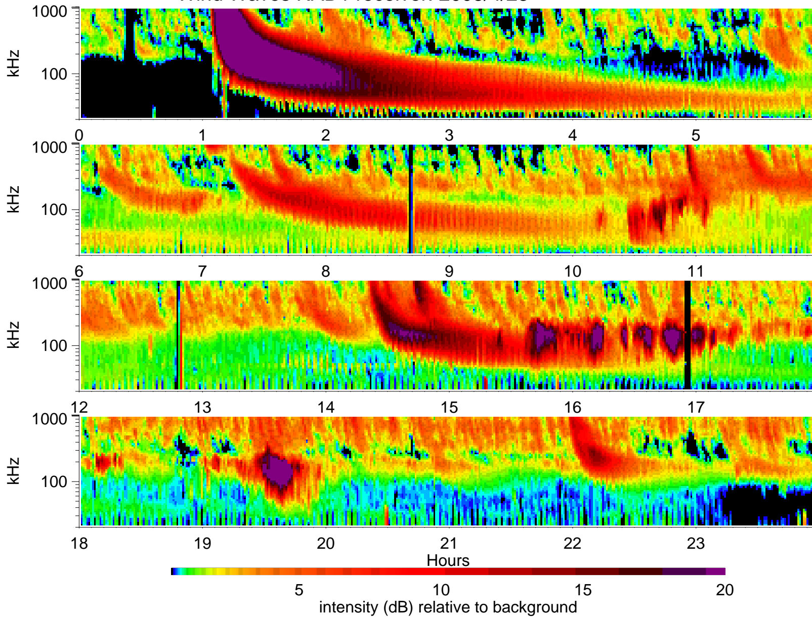
Wind Waves RAD1 receiver: 2003/4/23
