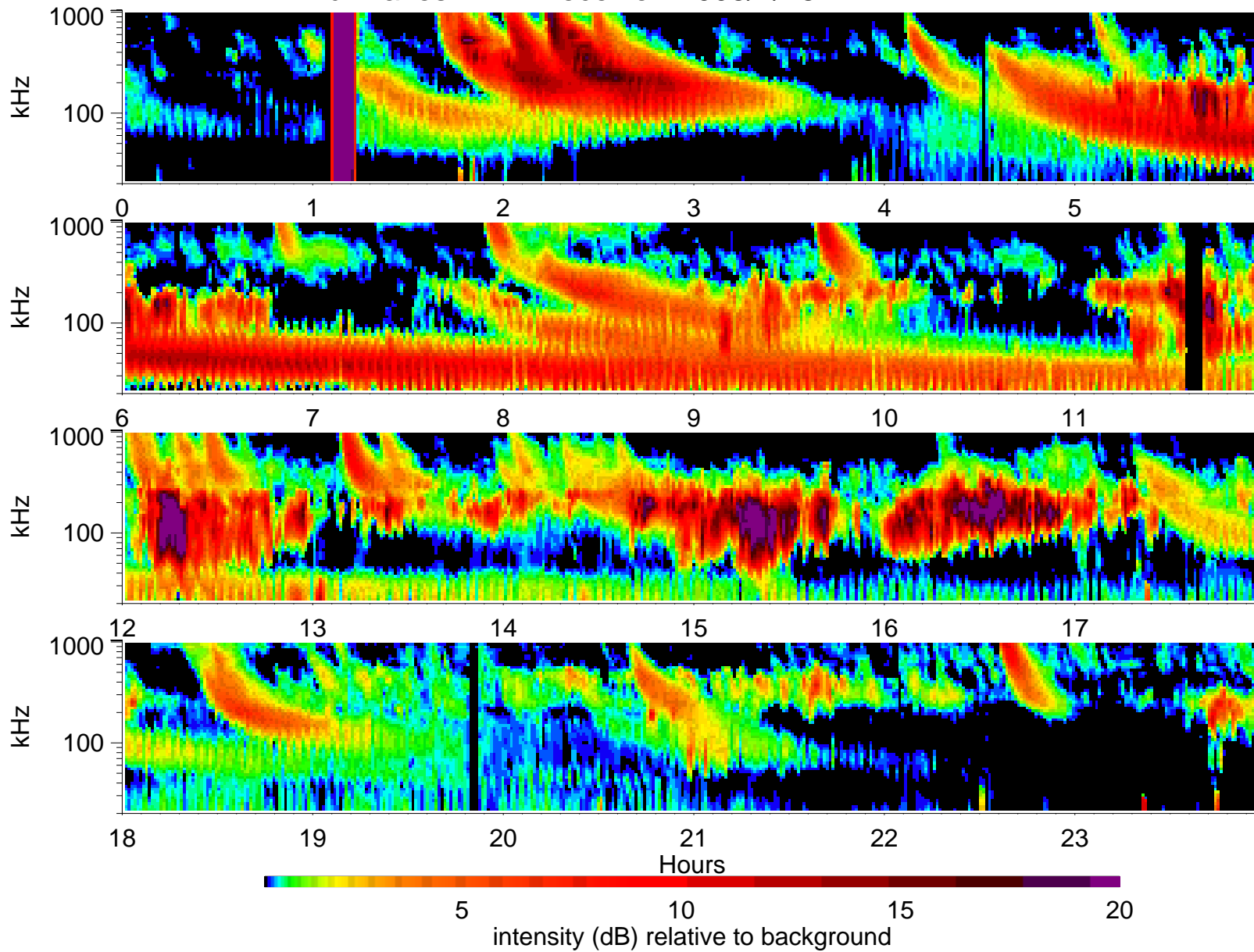
Wind Waves RAD1 receiver: 2003/4/18
