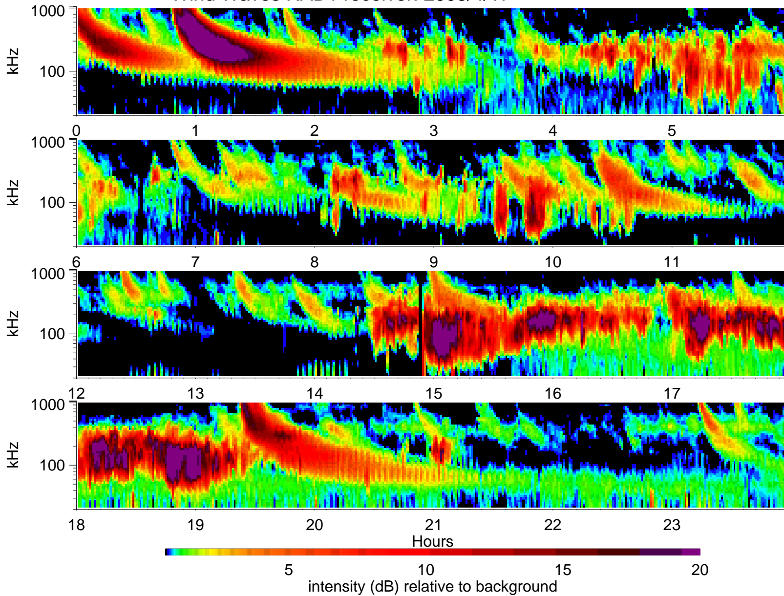
Wind Waves RAD1 receiver: 2003/4/17
