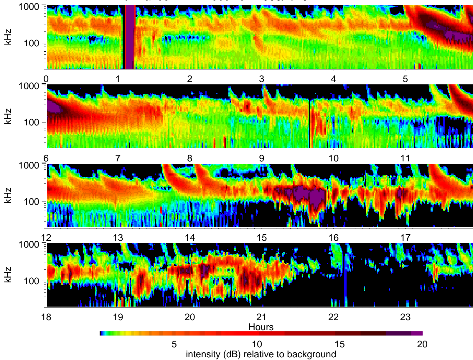
Wind Waves RAD1 receiver: 2003/4/16
