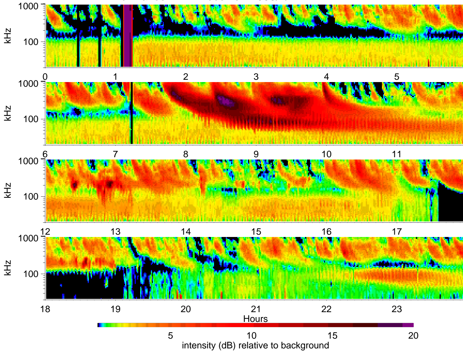
Wind Waves RAD1 receiver: 2003/4/14
