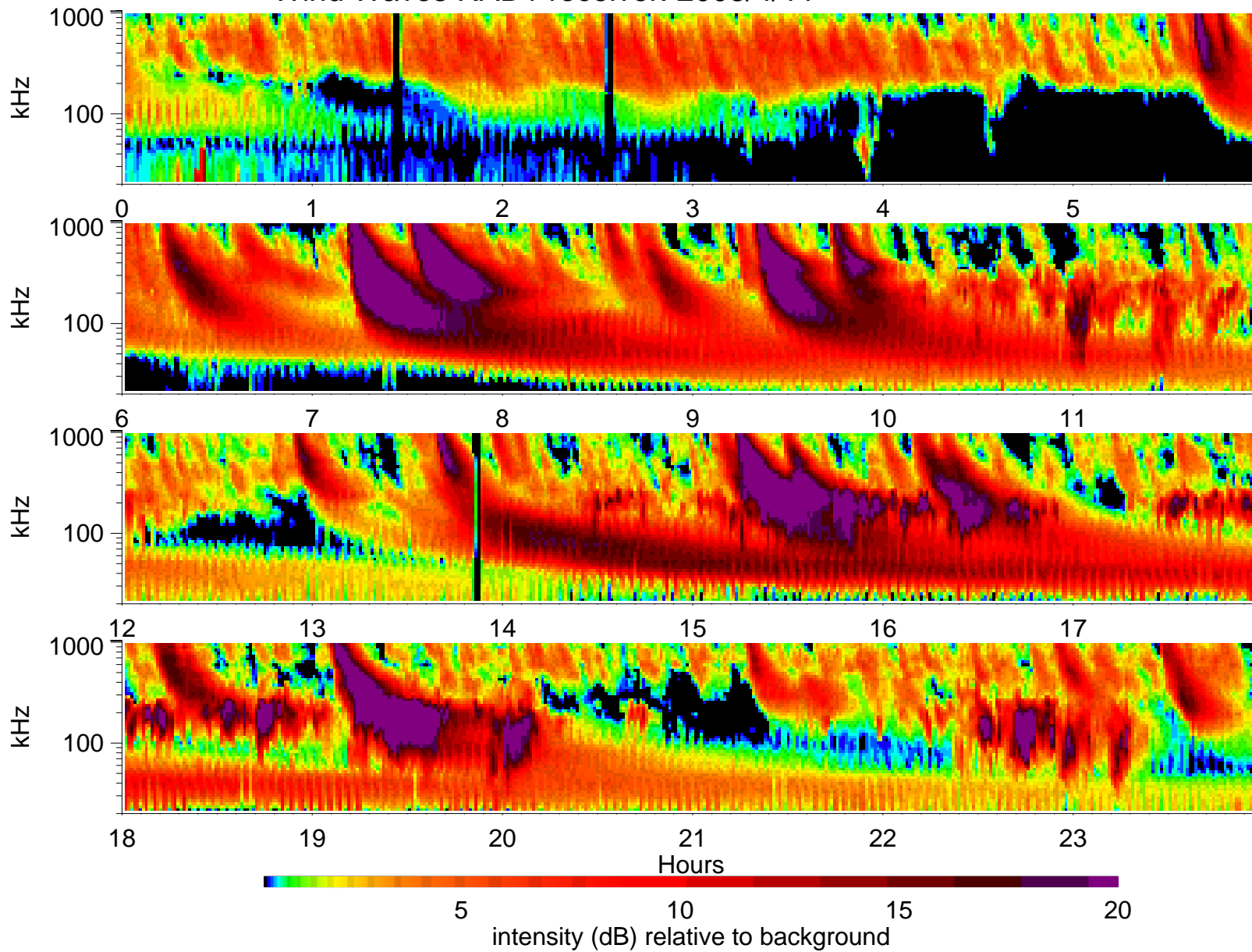
Wind Waves RAD1 receiver: 2003/4/11
