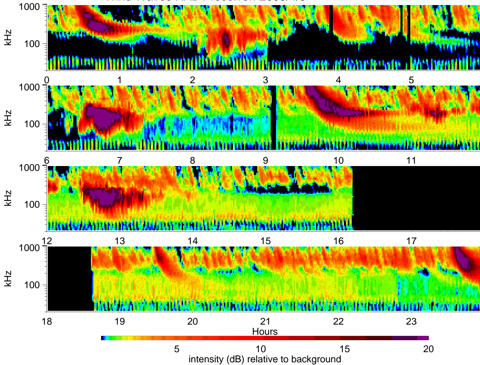
Wind Waves RAD1 receiver: 2003/4/9
