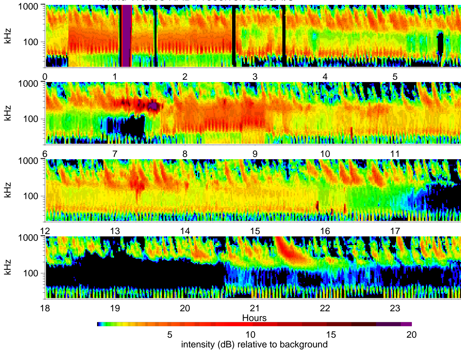
Wind Waves RAD1 receiver: 2003/4/8
