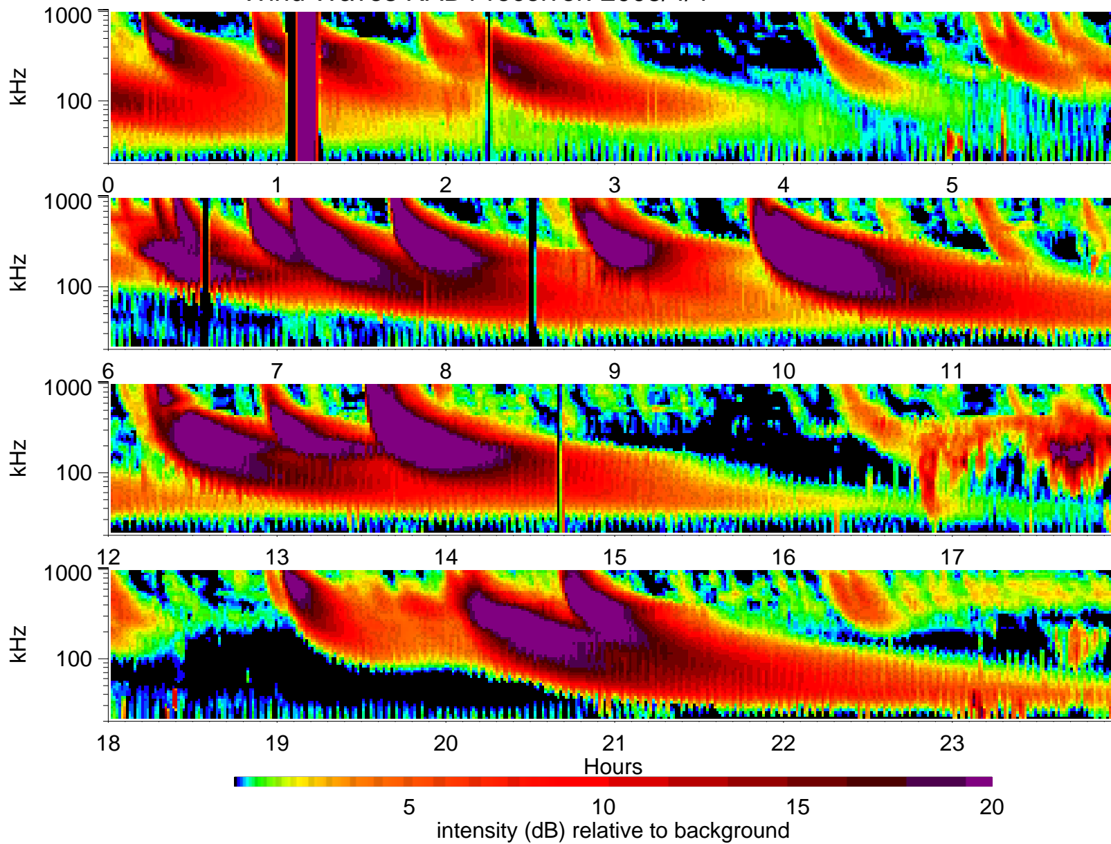
Wind Waves RAD1 receiver: 2003/4/4
