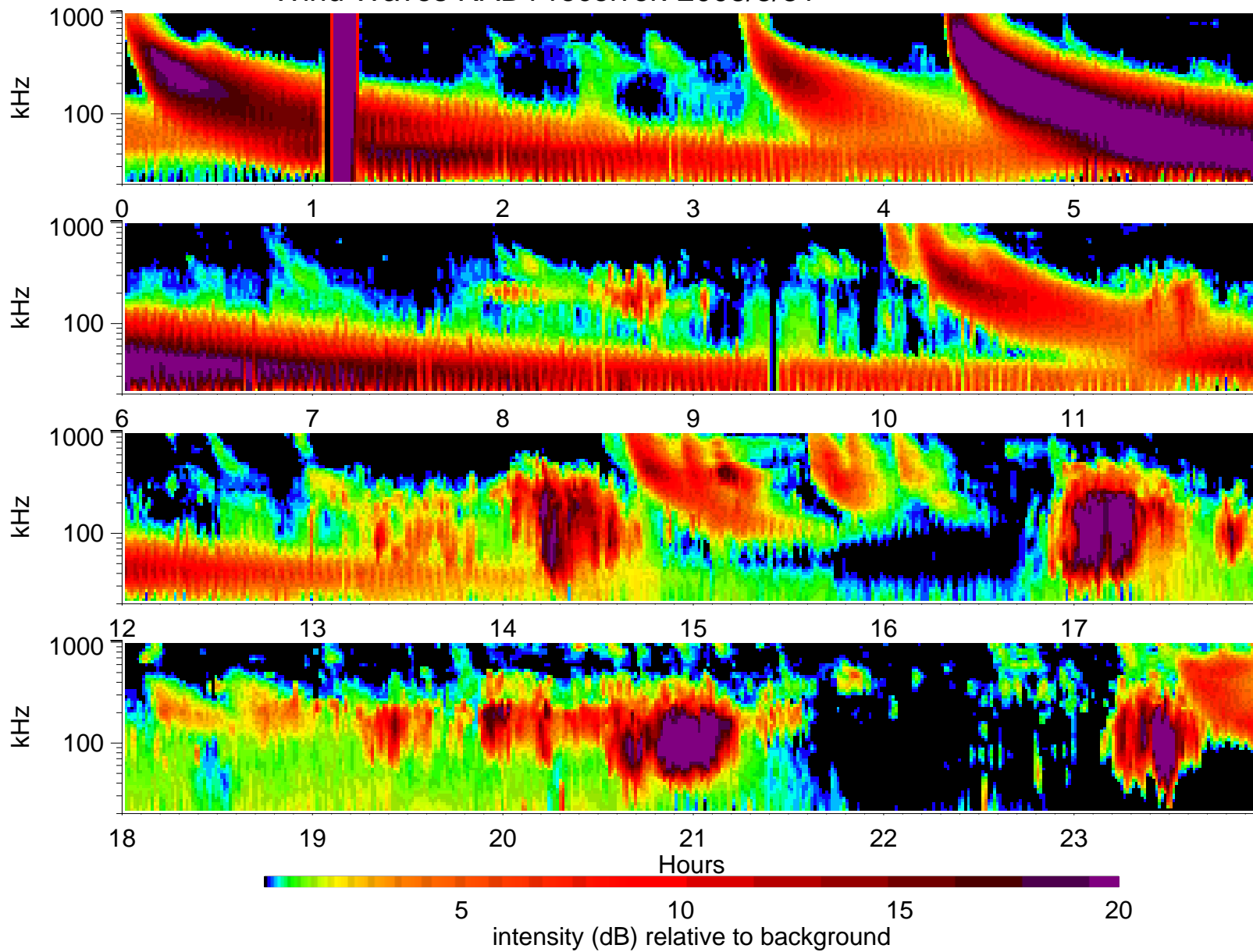
Wind Waves RAD1 receiver: 2003/3/31
