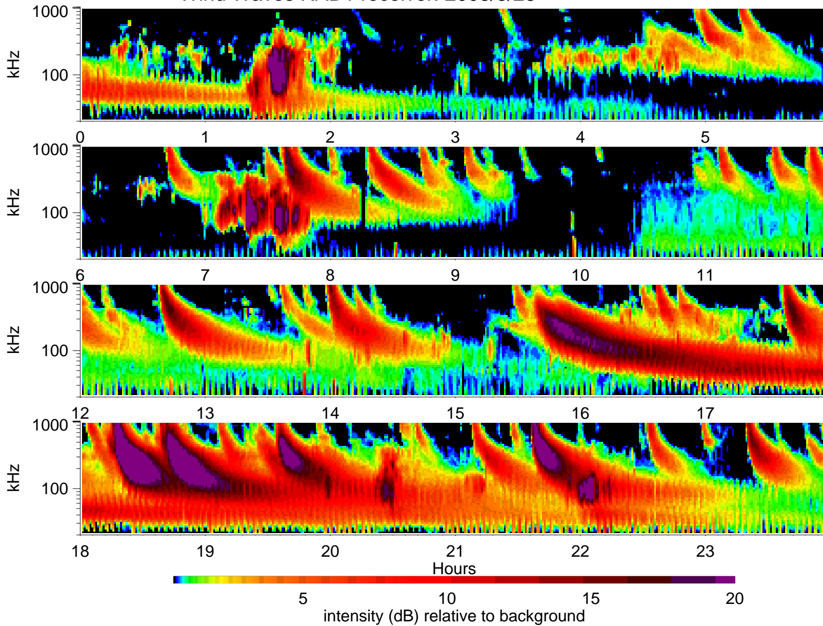
Wind Waves RAD1 receiver: 2003/3/28
