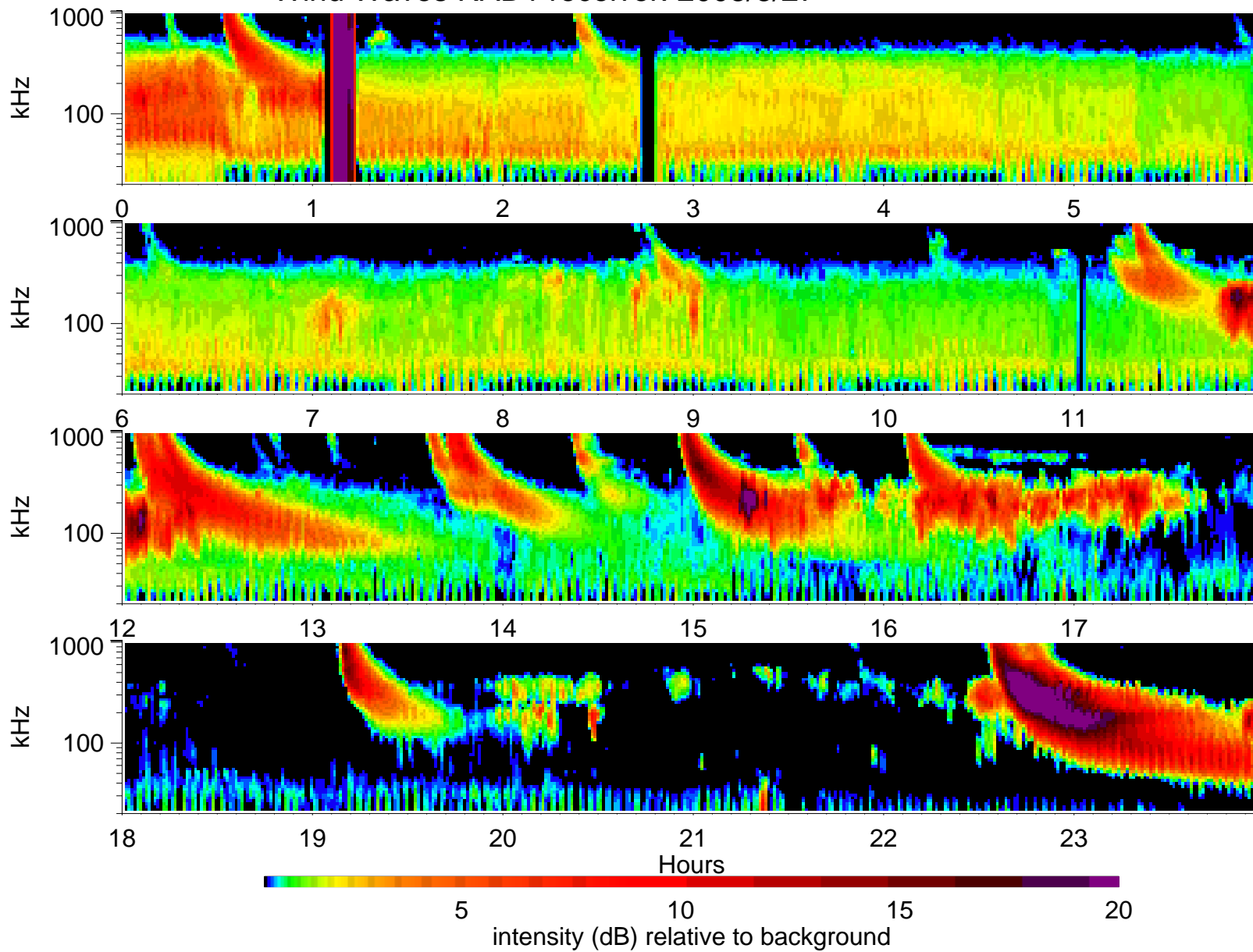
Wind Waves RAD1 receiver: 2003/3/27
