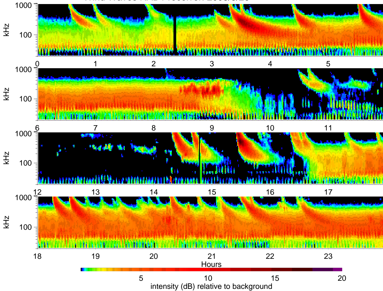
Wind Waves RAD1 receiver: 2003/3/26
