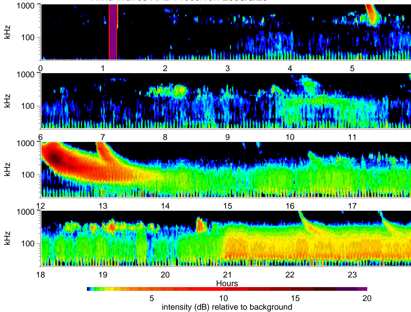
Wind Waves RAD1 receiver: 2003/3/25
