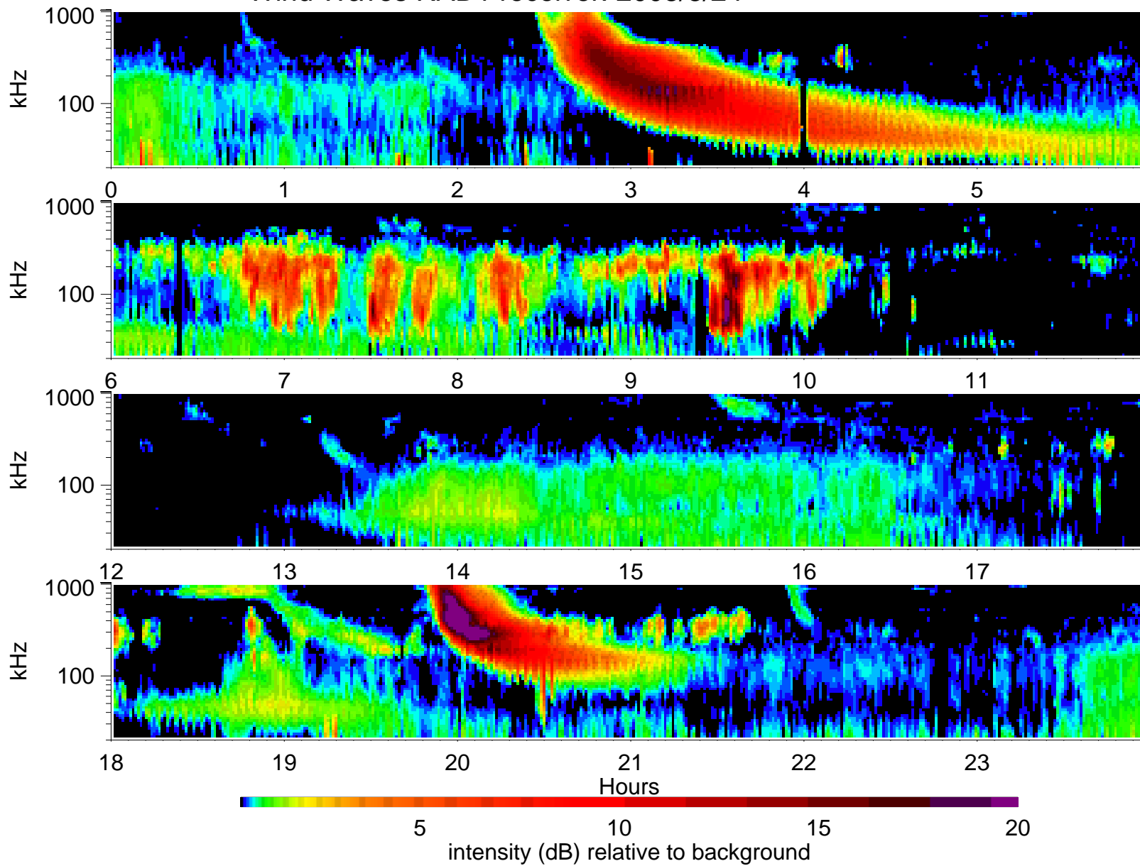
Wind Waves RAD1 receiver: 2003/3/24
