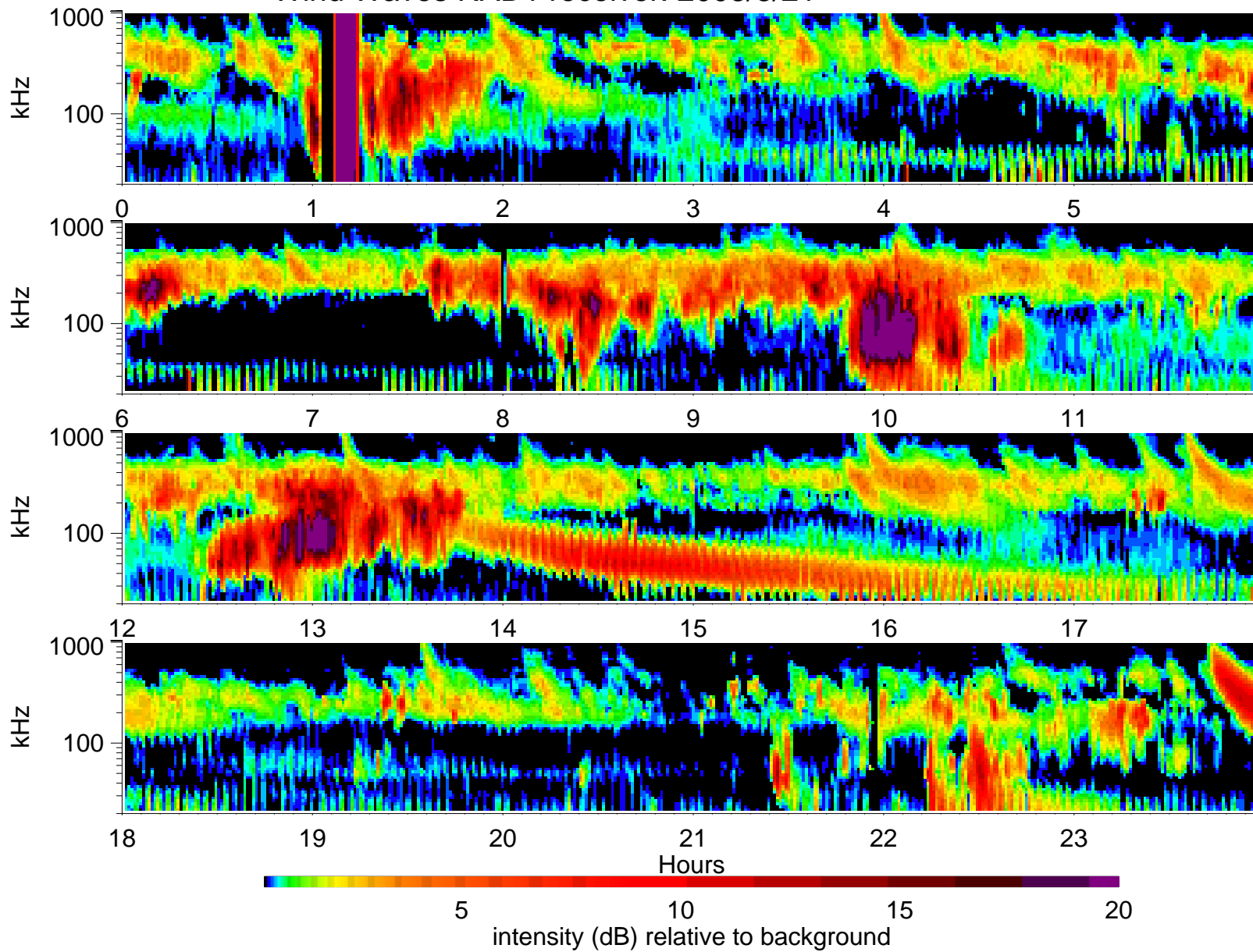
Wind Waves RAD1 receiver: 2003/3/21
