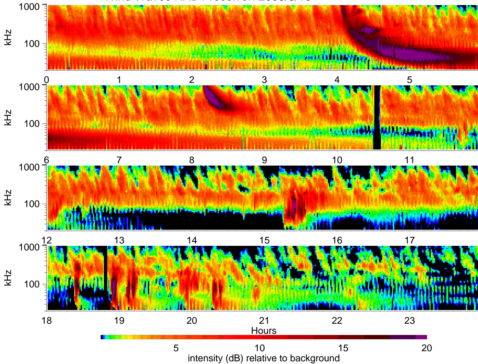
Wind Waves RAD1 receiver: 2003/3/16
