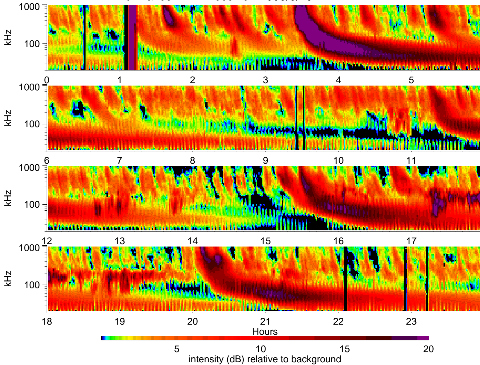
Wind Waves RAD1 receiver: 2003/3/15
