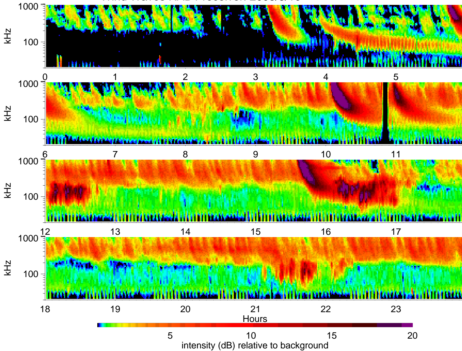
Wind Waves RAD1 receiver: 2003/3/10
