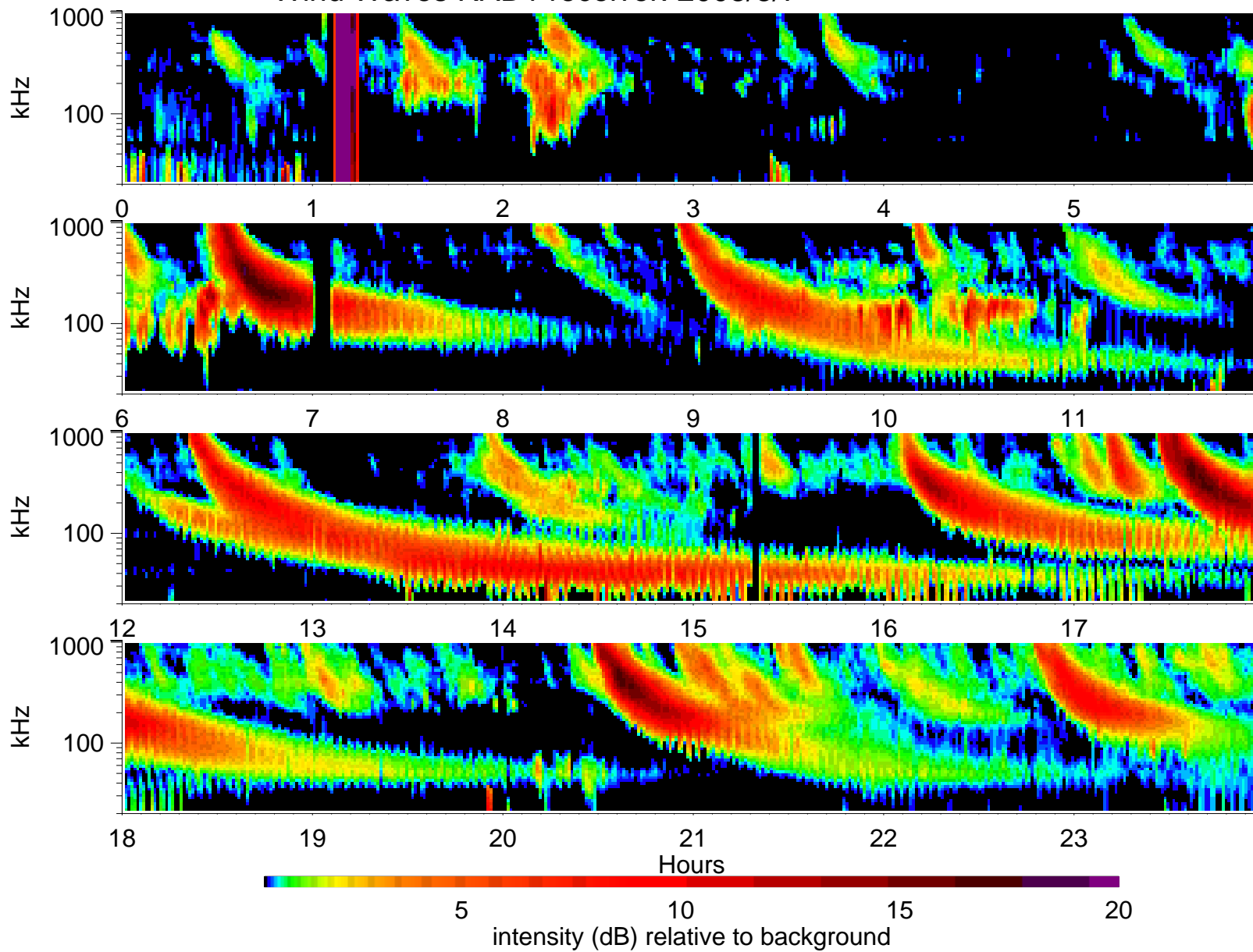
Wind Waves RAD1 receiver: 2003/3/7
