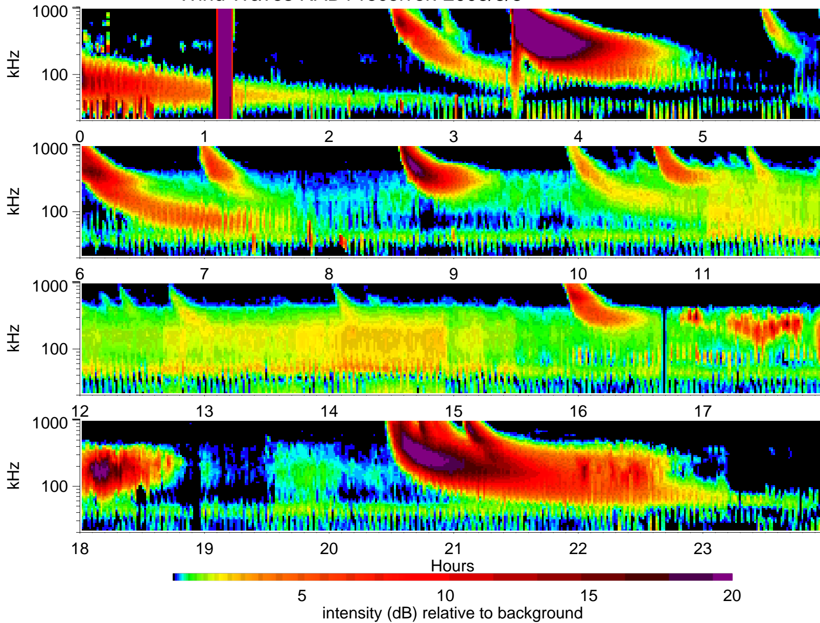
Wind Waves RAD1 receiver: 2003/3/3
