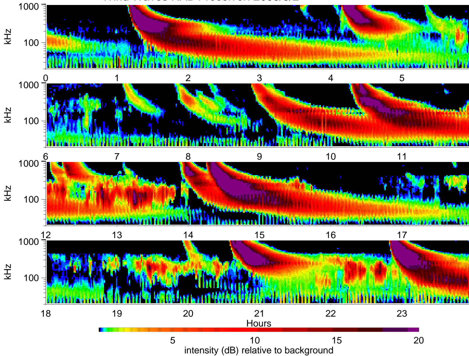
Wind Waves RAD1 receiver: 2003/3/2
