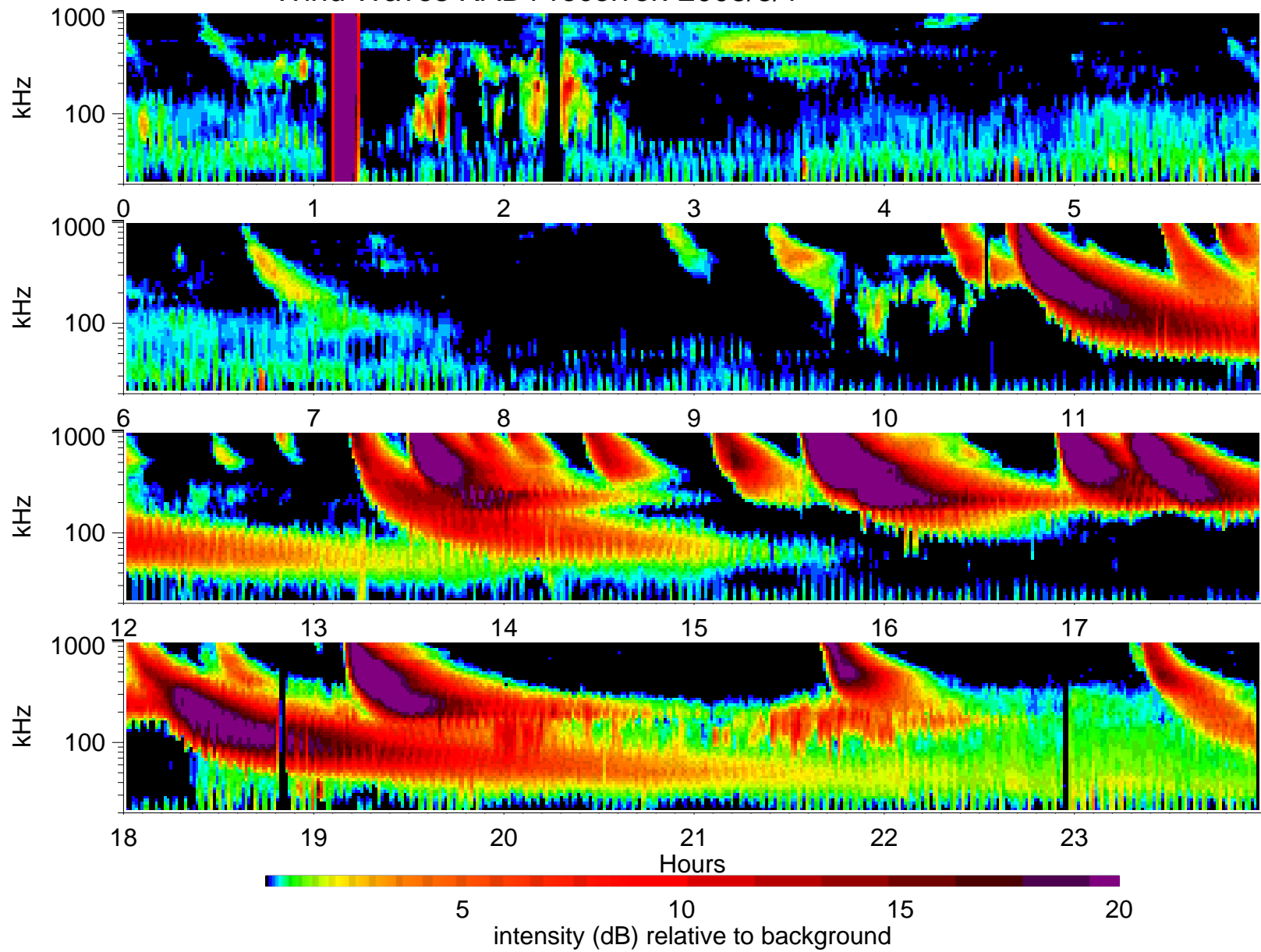
Wind Waves RAD1 receiver: 2003/3/1
