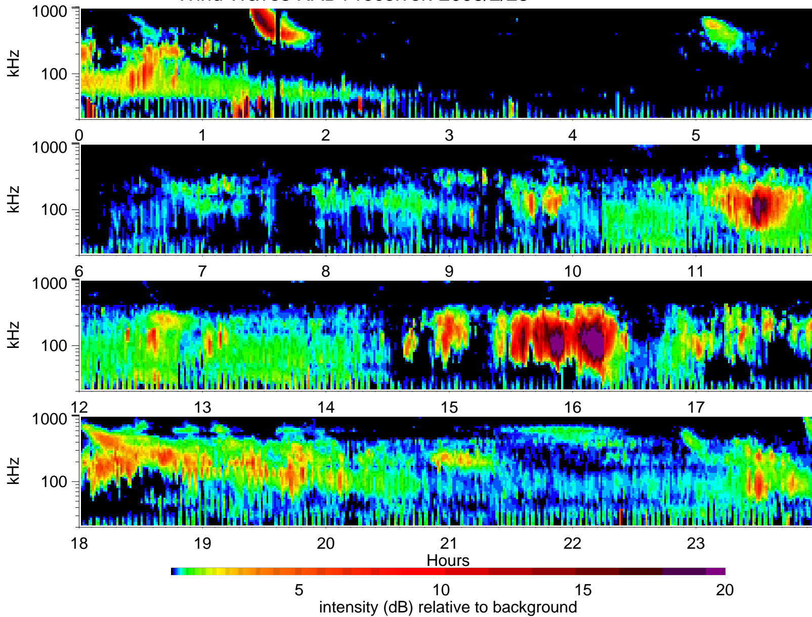
Wind Waves RAD1 receiver: 2003/2/28
