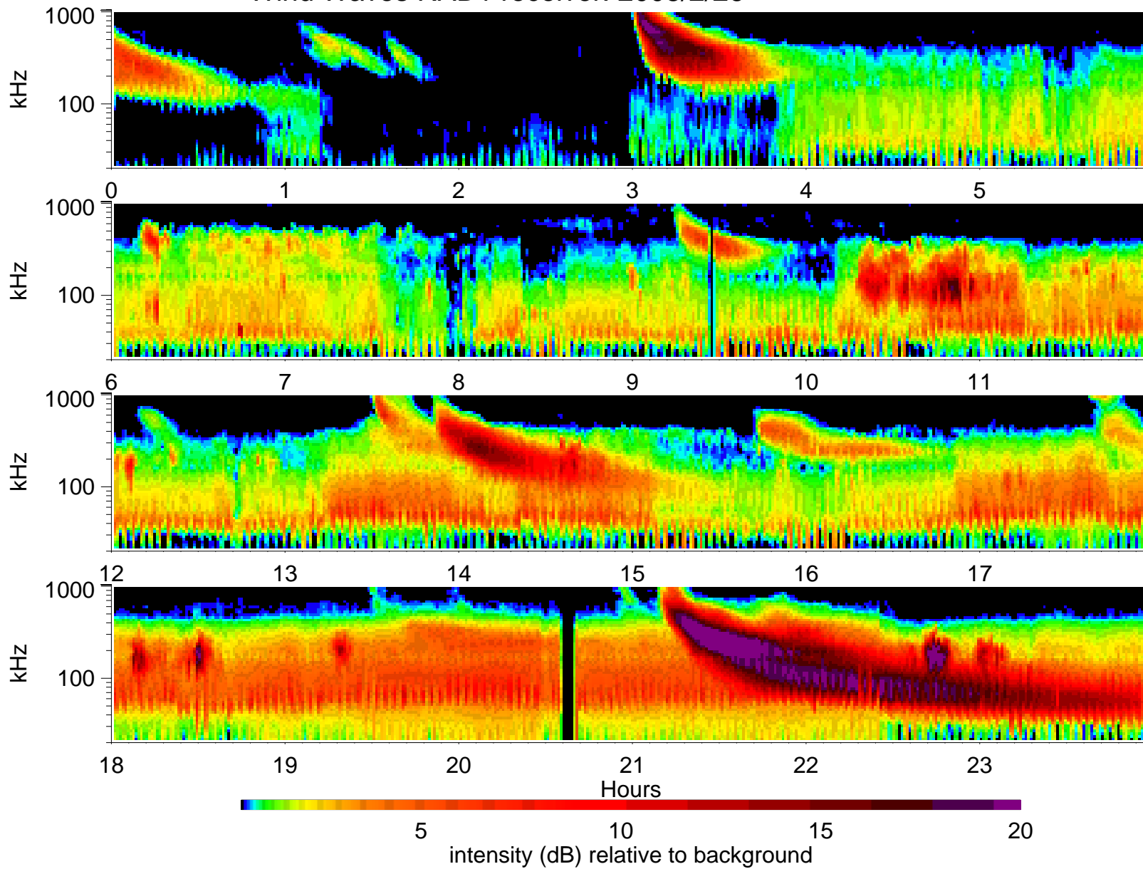
Wind Waves RAD1 receiver: 2003/2/26
