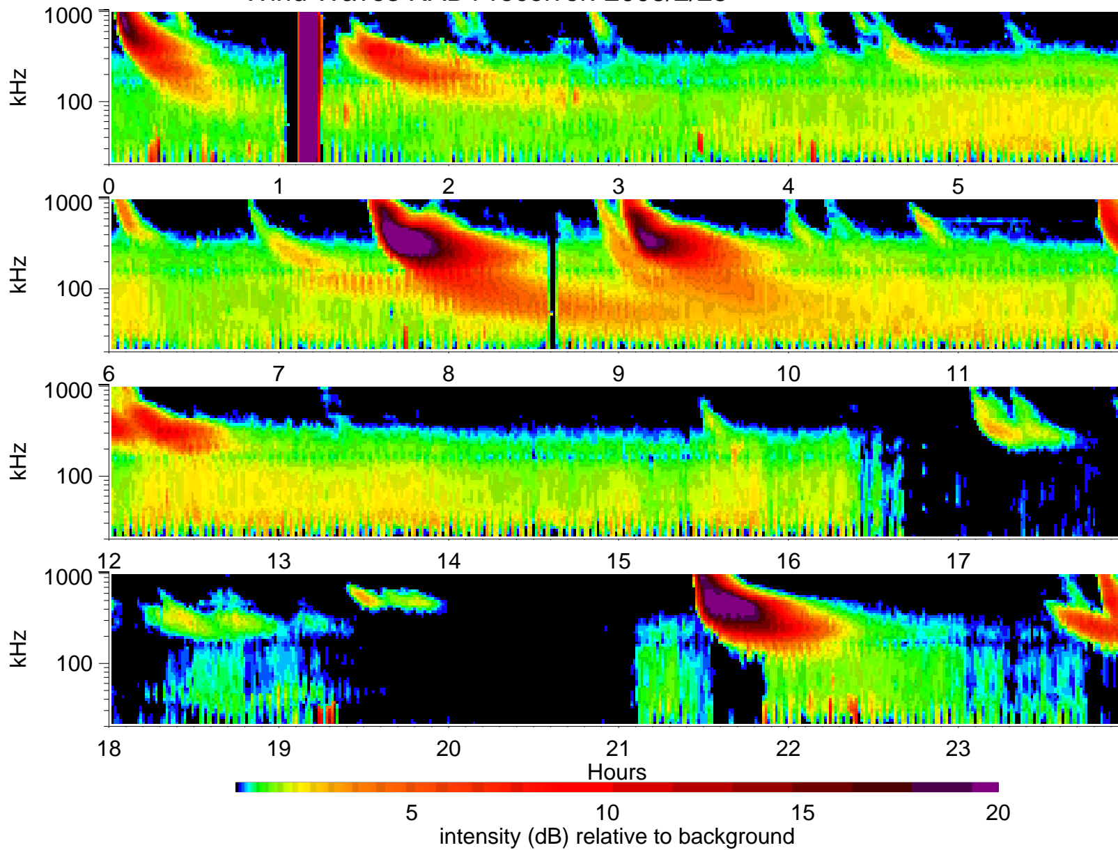
Wind Waves RAD1 receiver: 2003/2/25
