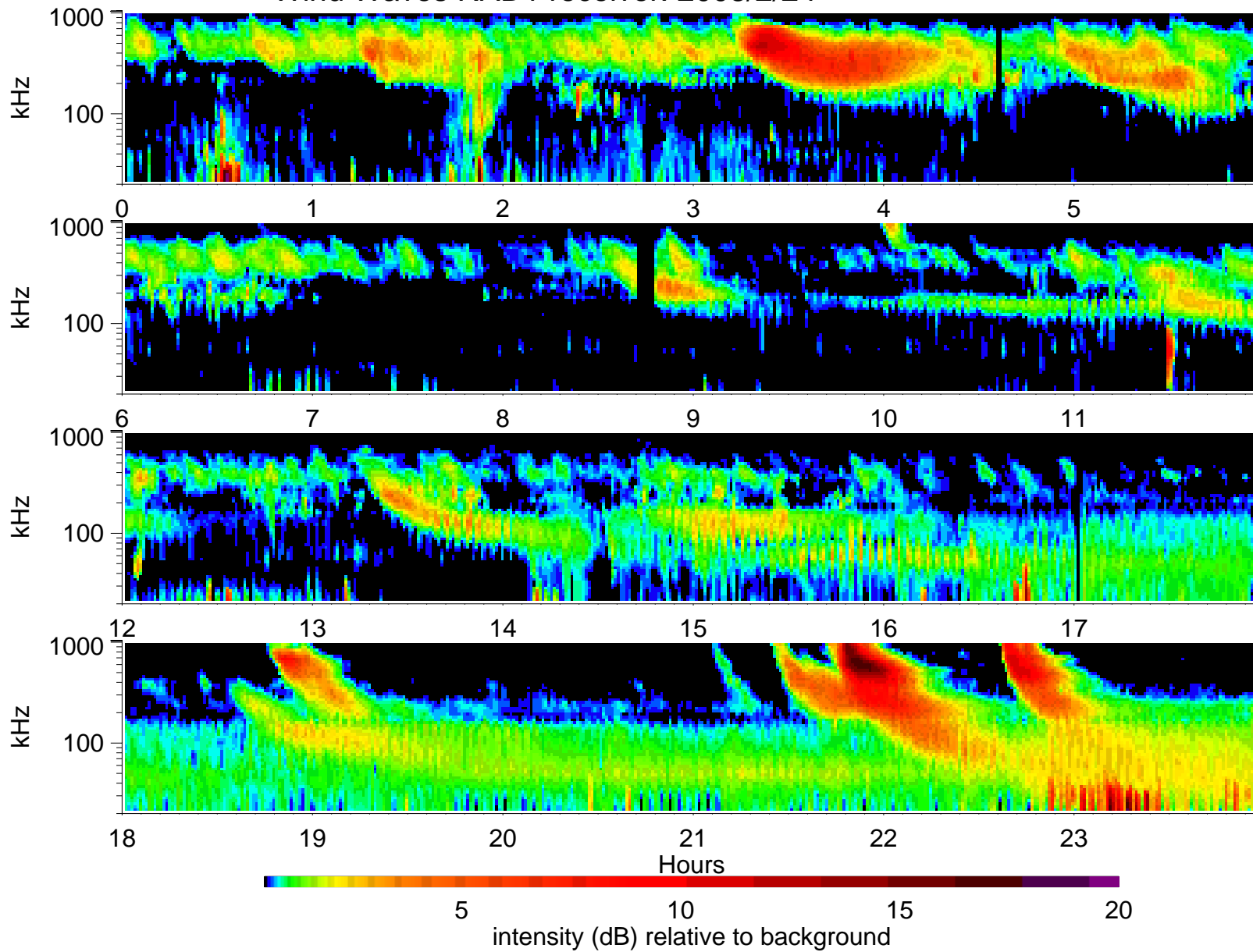
Wind Waves RAD1 receiver: 2003/2/24
