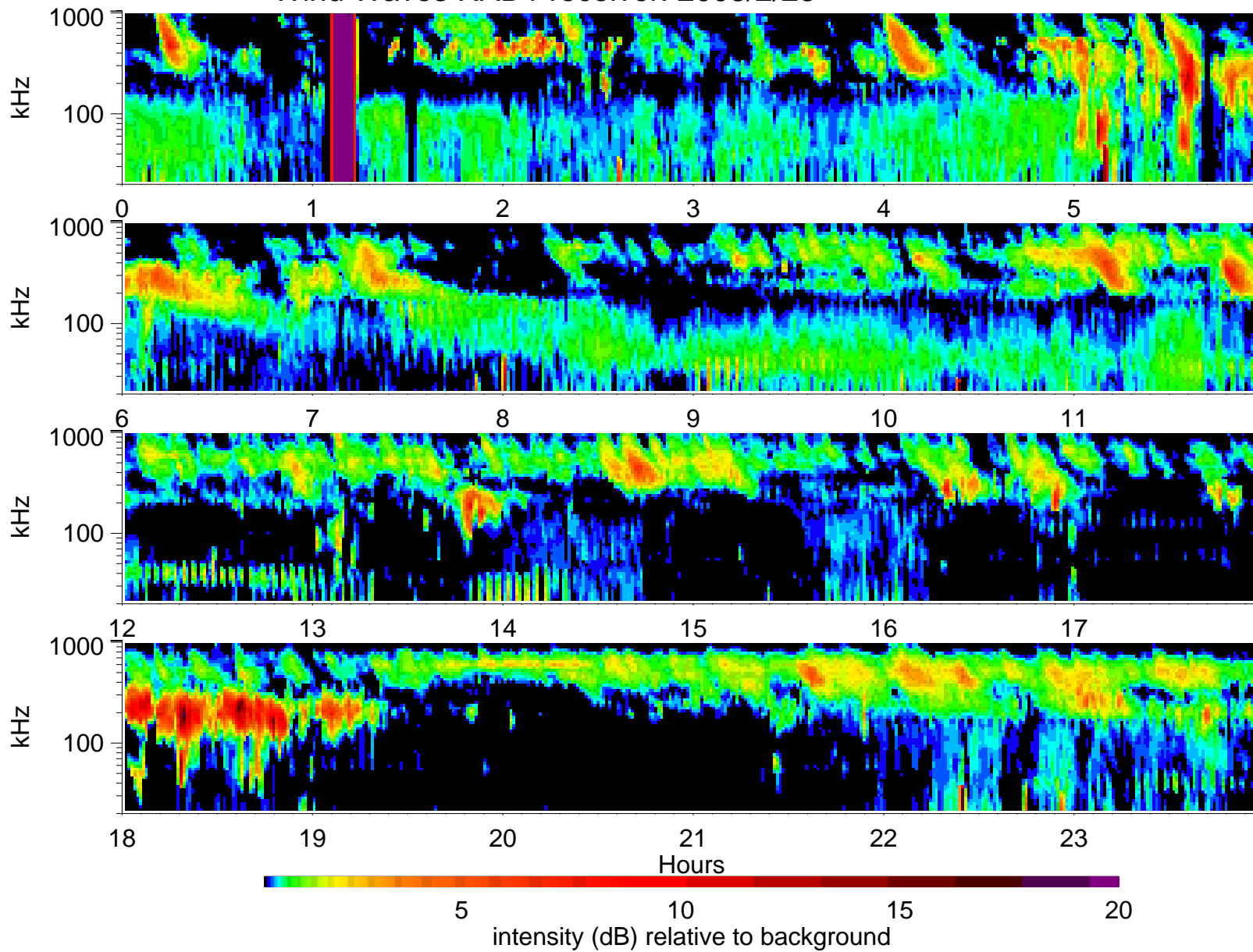
Wind Waves RAD1 receiver: 2003/2/23
