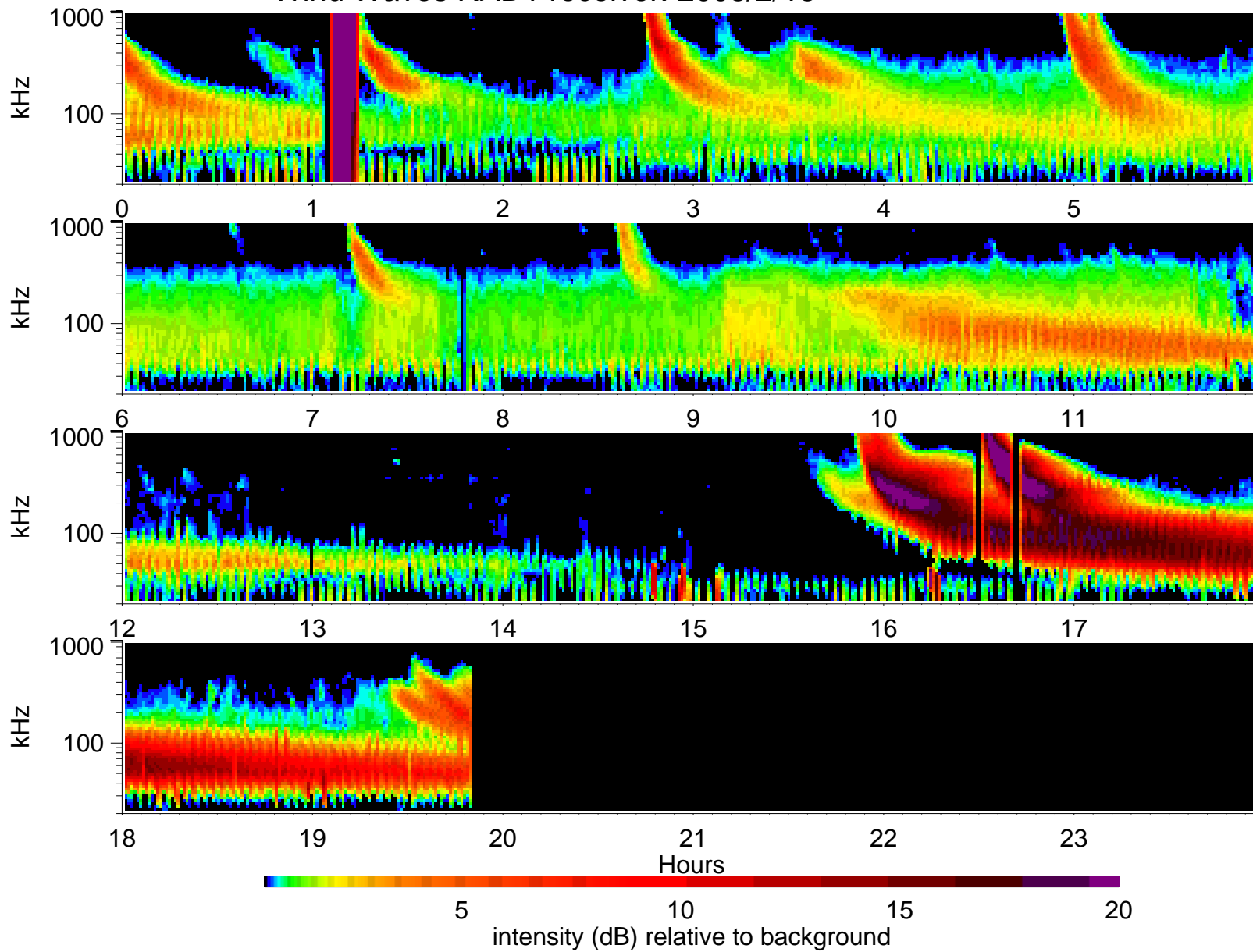
Wind Waves RAD1 receiver: 2003/2/13
