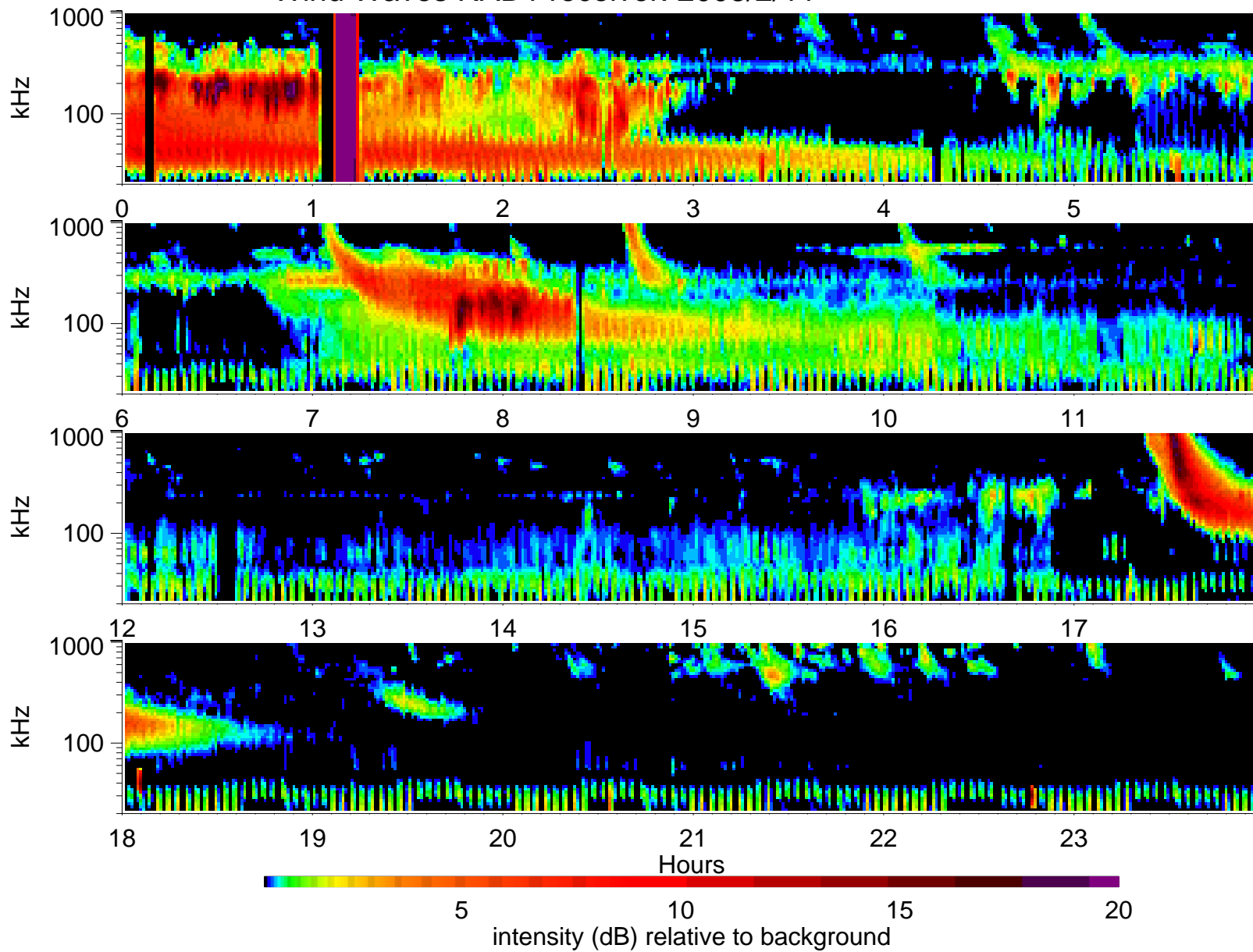
Wind Waves RAD1 receiver: 2003/2/11
