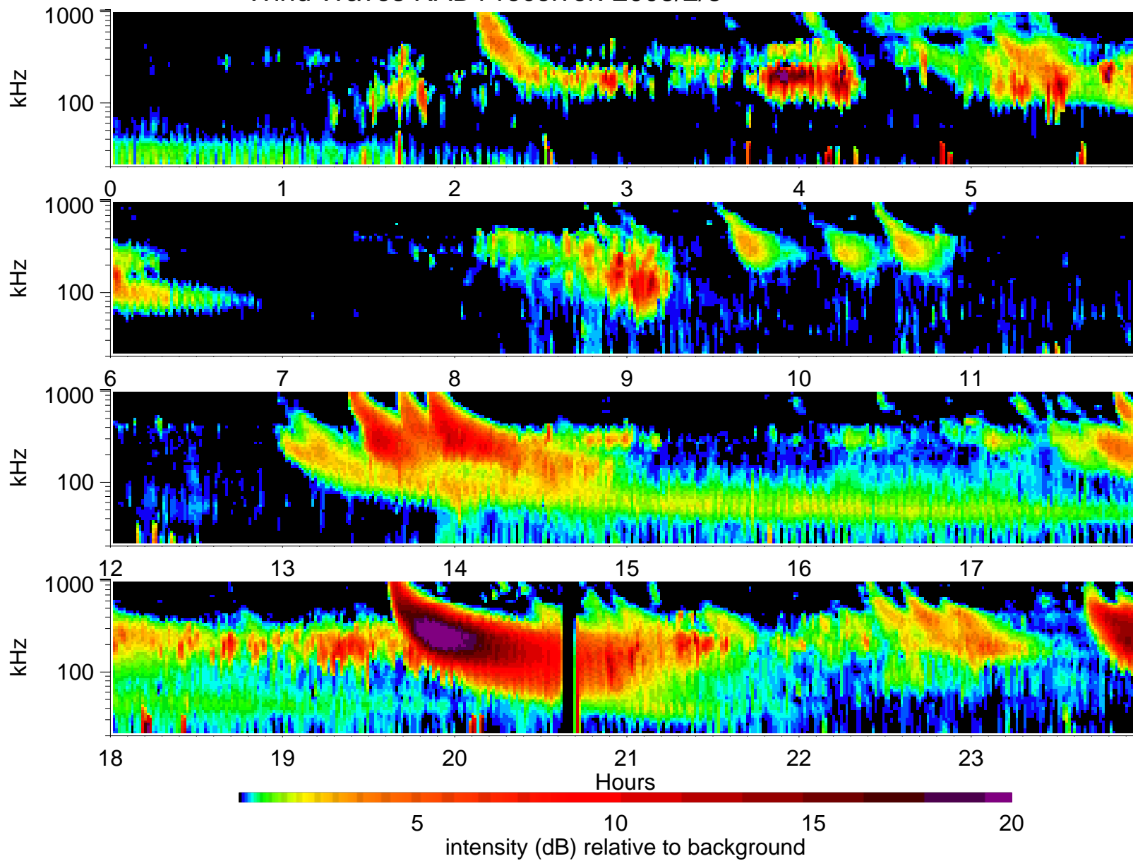
Wind Waves RAD1 receiver: 2003/2/8
