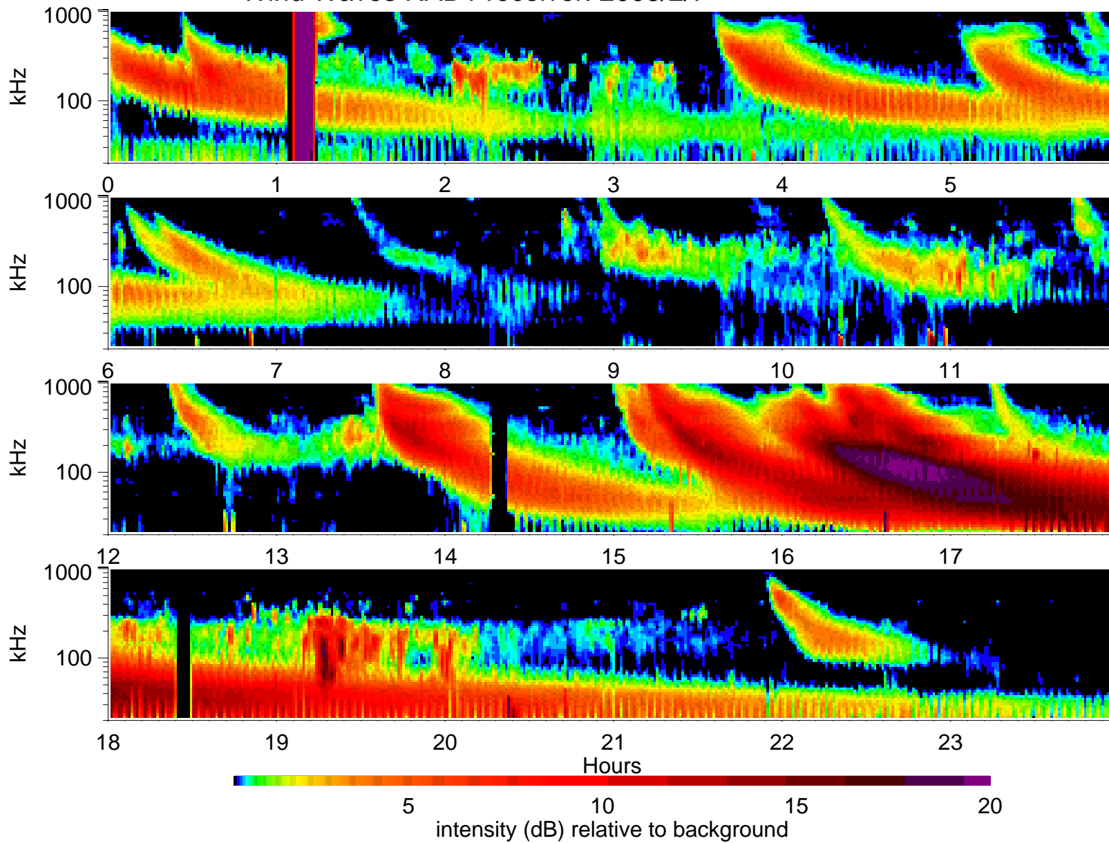
Wind Waves RAD1 receiver: 2003/2/7
