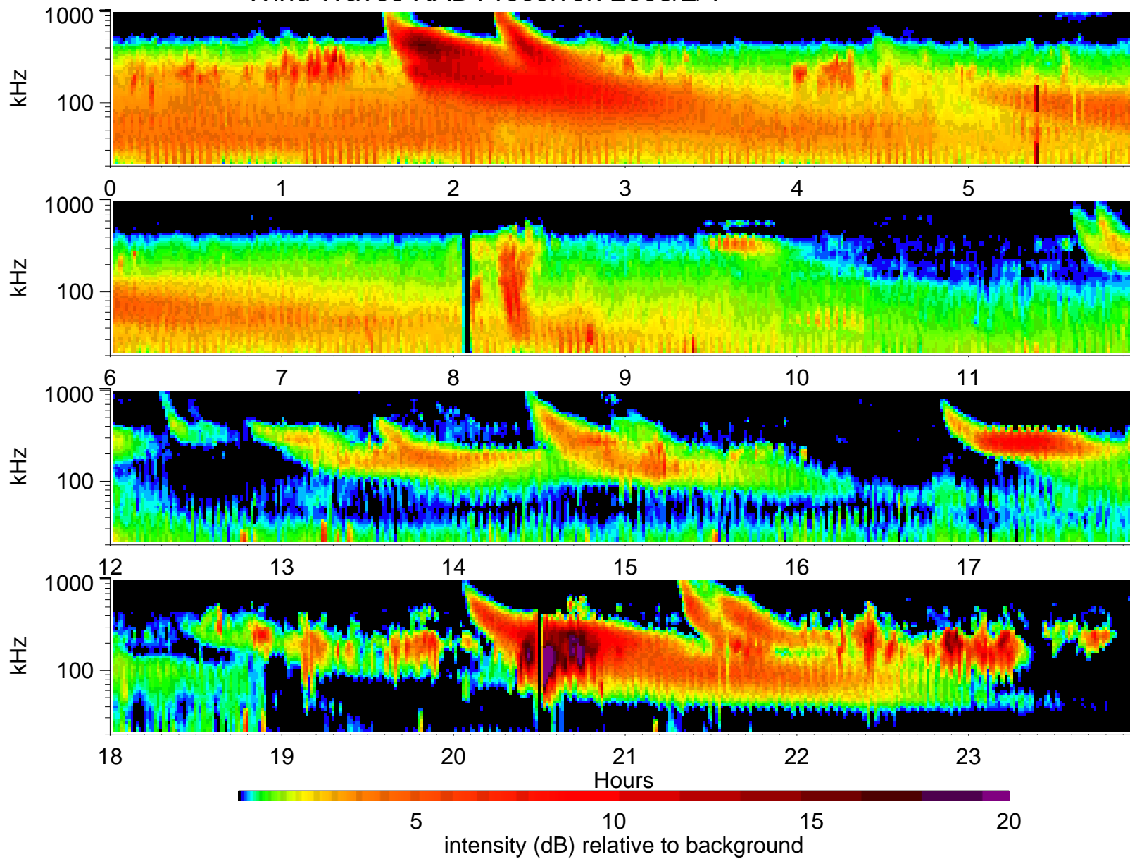
Wind Waves RAD1 receiver: 2003/2/4
