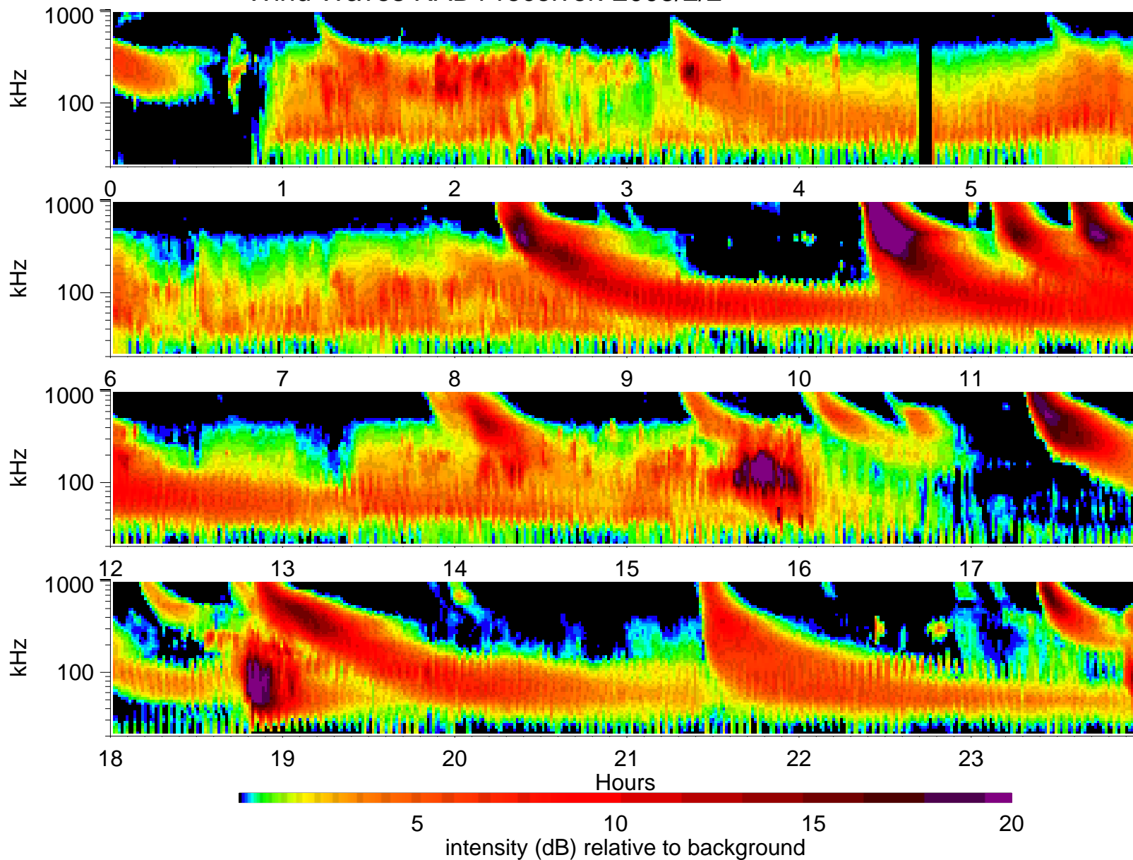
Wind Waves RAD1 receiver: 2003/2/2
