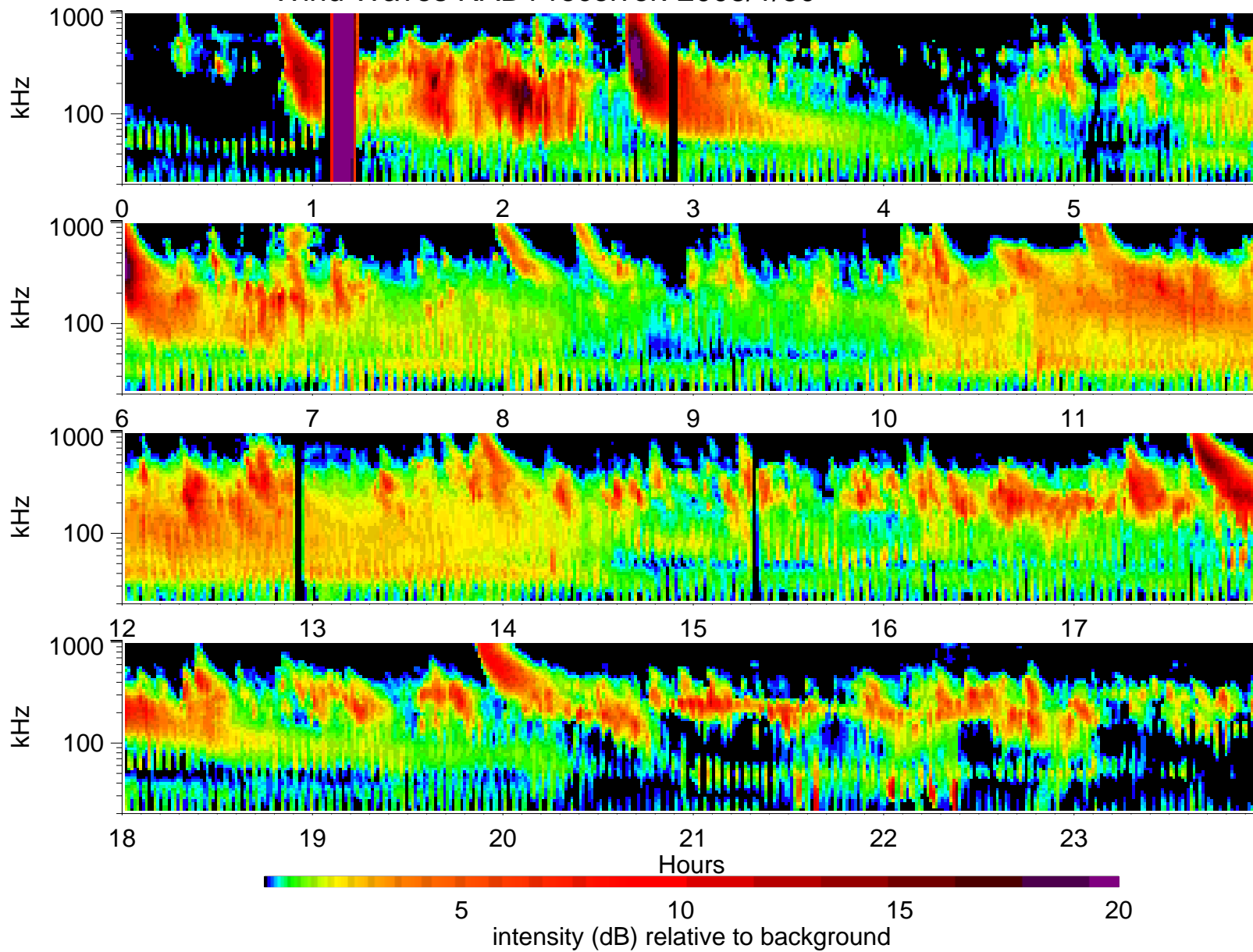
Wind Waves RAD1 receiver: 2003/1/30
