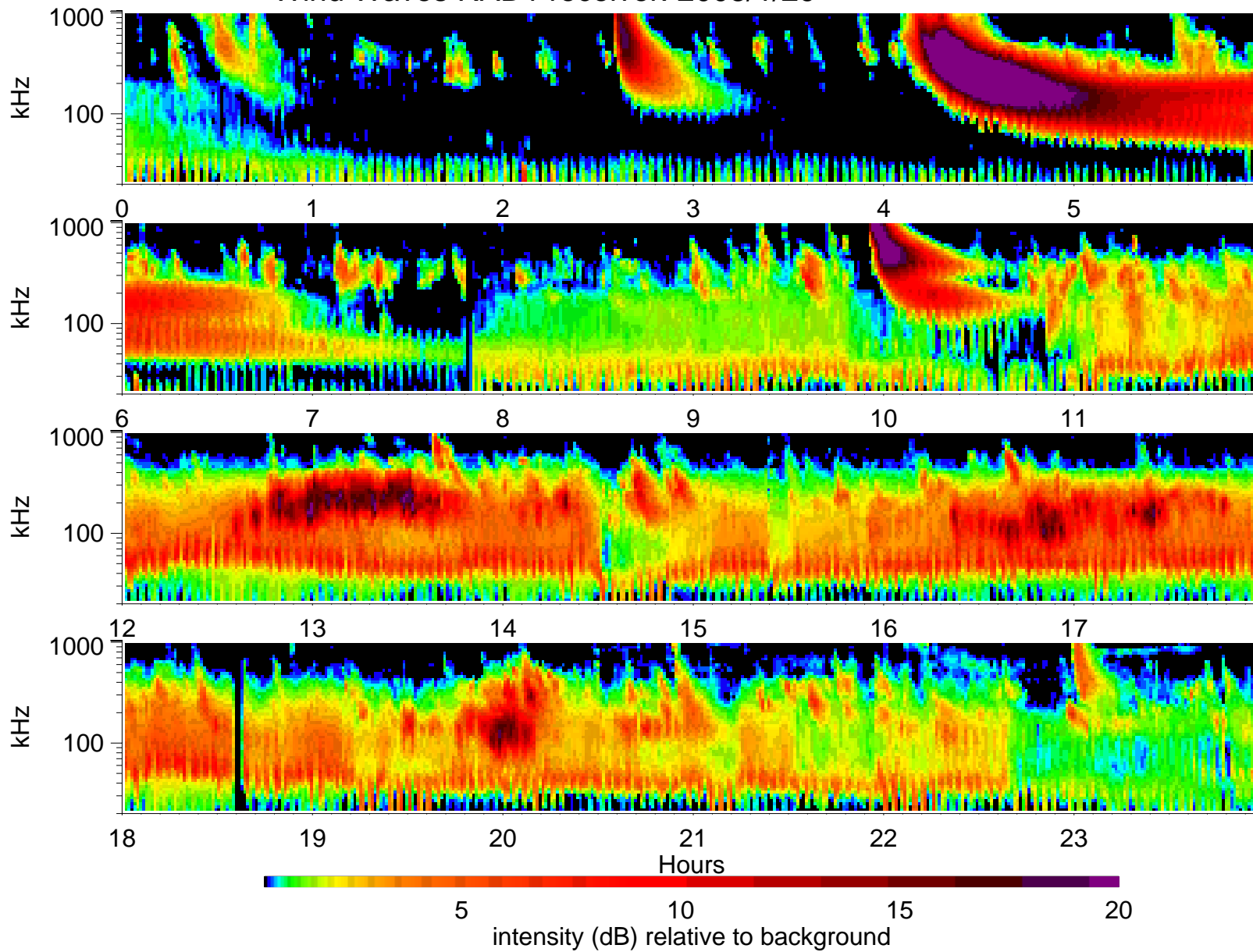
Wind Waves RAD1 receiver: 2003/1/29
