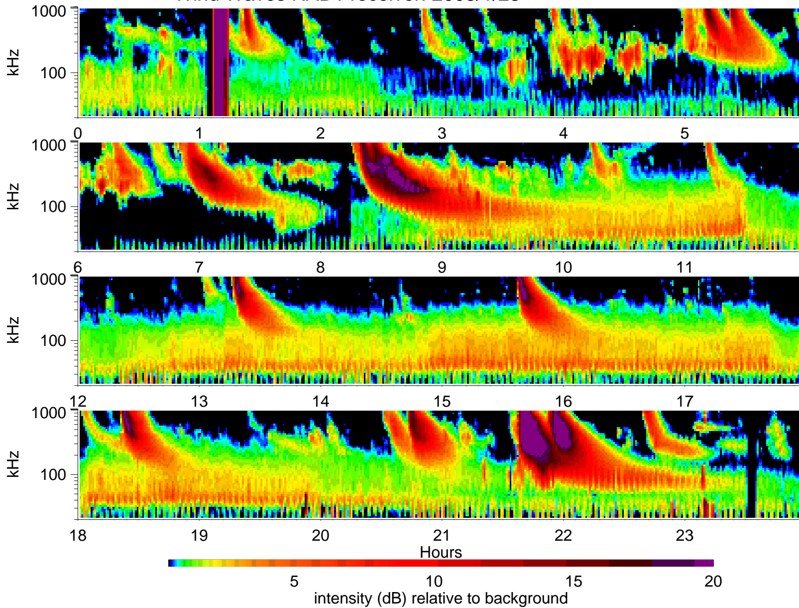
Wind Waves RAD1 receiver: 2003/1/28
