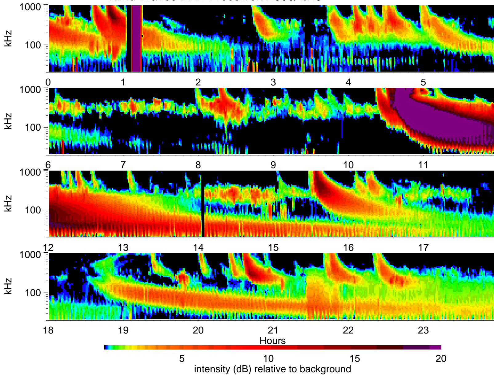
Wind Waves RAD1 receiver: 2003/1/26
