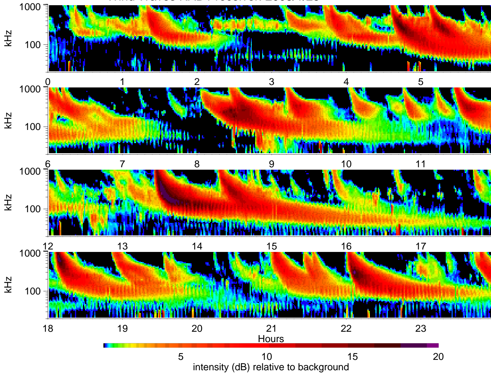
Wind Waves RAD1 receiver: 2003/1/25
