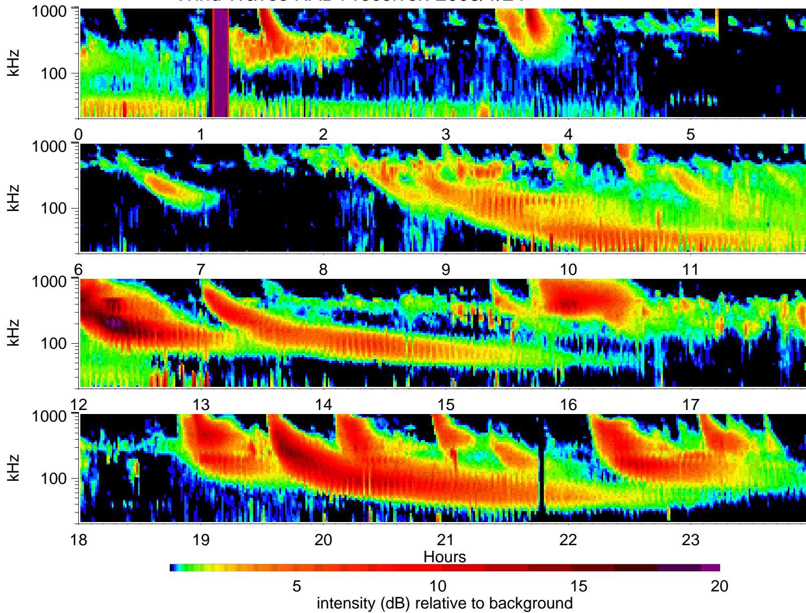
Wind Waves RAD1 receiver: 2003/1/24
